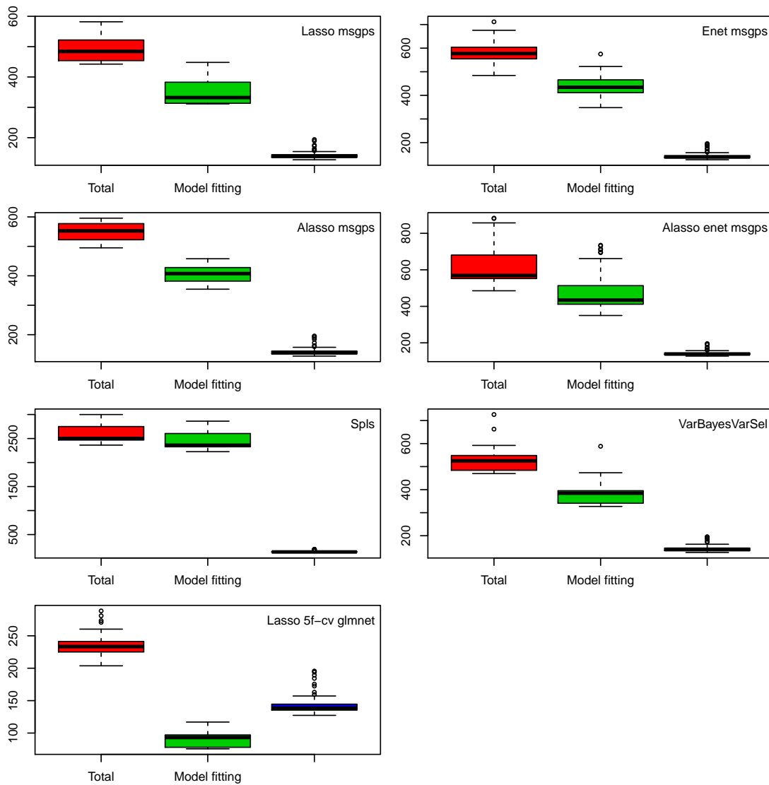
Figure 5.9 : Timing of SelectBoost for the seven linear regression models and Type 1 datasets.
