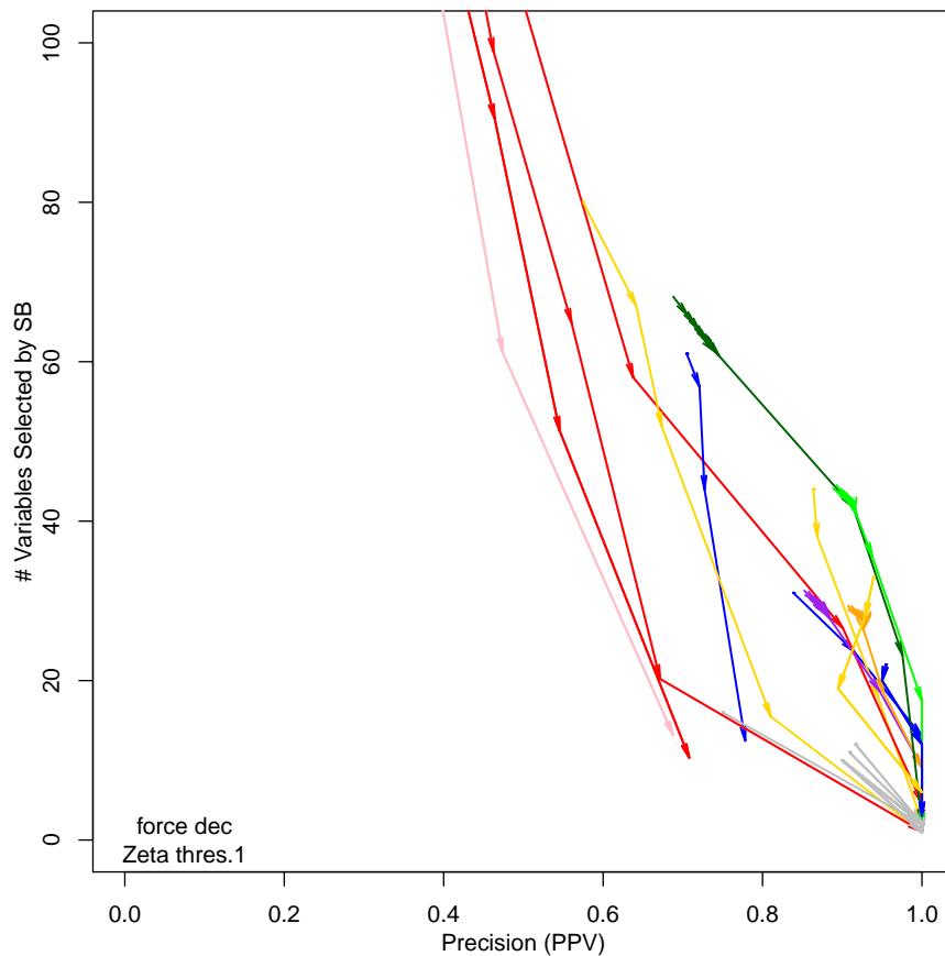
Figure 5.3 : The average number of identified variables is plotted as a function of the proportion of correctly identified variables for Type1 simulated data and all models.
