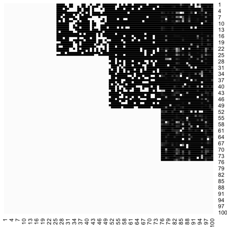
Figure 5.7 : Post inference analysis of an inferred cascade network. Dark values are tantamount to low confidence. Bright values are tantamount to high confidence. Confidence ranges from 0 (lowest) to 1 (highest). The lower triangular part of the matrix is an area with the highest confidence (1) since we know -and assume so in the model- that for cascade networks those links must be equal to 0.
