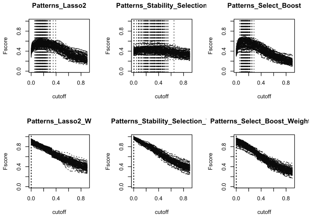
Figure 5.8 : F -score as a function of the thresholding value: if an inferred coefficient for the network is less than the thresholding value, then it is set to 0. The SelectBoost algorithm is compared to both stability selection and the regular lasso. The upper row displays results for the unweighted version of the algorithms, whereas the lower row displays results for their weighted counterparts.
