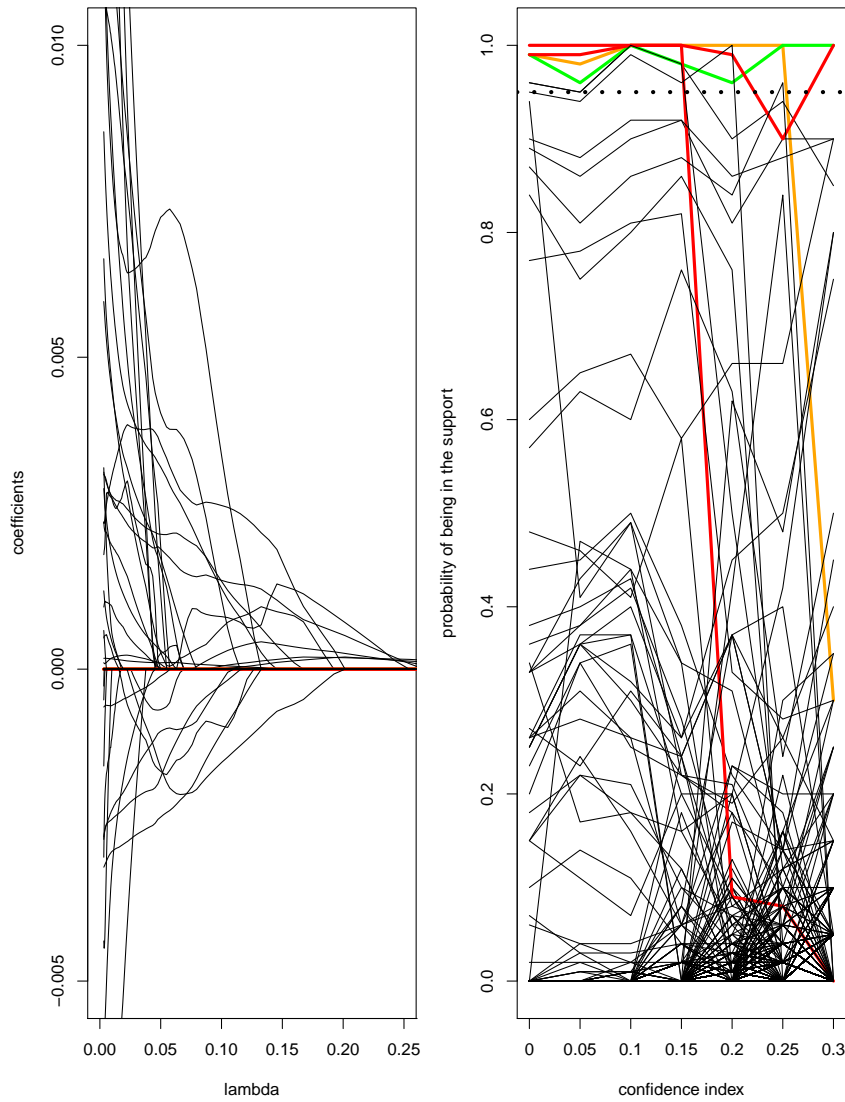
Figure 5.6 : Colors: the green is for the most reliable variables selected by the SelectBoost algorithm (confidence index of 0.3; orange is for intermediate confidence (0.25) and red for low confidence (0.15)). Left: evolution of the coefficients in the lasso regression when the regularization parameter \lambda is varying. Right: evolution of the probability of being in the support of the regression when the confidence index is varying. The dotted line represents the threshold of 0.95.
