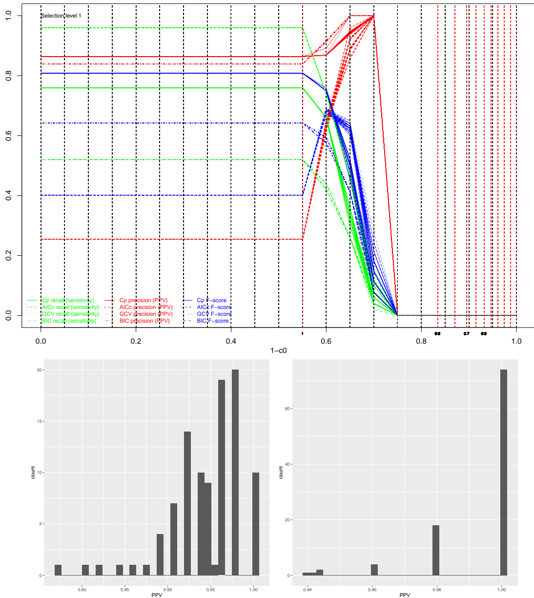
Figure 5.1 : Top: evolution of the recall, PPV and F-score as a function of 1 - c_0 for LASSO-based SelectBoost for Type1 simulated data with a non-increasing post-processing step . Bottom: the distribution of the PPV for a 0.25 threshold and c_0 = \text{mean}(q_{90}, q_{100}) for SPLS-based SelectBoost and Type1 data.
