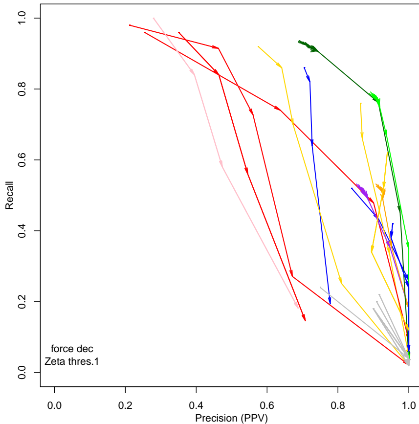
Figure 5.2 : Recall-precision curve. All models and criteria non-increasing SelectBoost. Type 1 data. Direct grouping. 100 different datasets. \zeta_{\min} = 1
