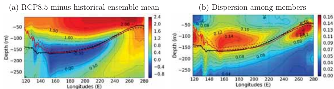
Figure 5.5 – Changes in vertical stratification in CESM-LE. (5.5a) Differences between ensemble-mean RCP8.5 minus historical equatorial ( 2^{\circ}\text{S}-2^{\circ}\text{N} ) temperature anomalies ( ^{\circ}\text{C} ). (5.5b) Dispersion among the ensemble of the mean temperature difference ( ^{\circ}\text{C} ). Red lines indicate the ensemble-mean depth of the thermocline defined as the depth of the maximum value of the vertical temperature gradient. Black line are the ensemble-mean depth of the 20^{\circ}\text{C} isotherm. Solid lines are for the ensemble-mean of CESM-LE historical simulations and dashed lines are for the ensemble-mean of RCP8.5 simulations.
