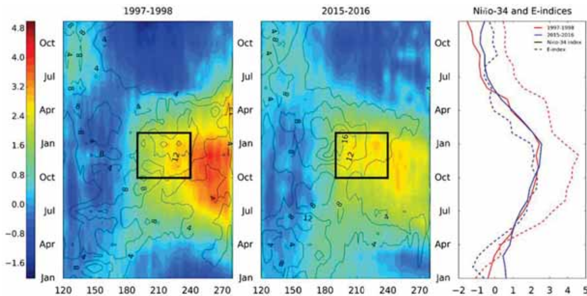
Figure 1.5 – Time-longitude sections of the equatorial band ( 2^{\circ}\text{S}-2^{\circ}\text{N} ) SST anomalies ( ^{\circ}\text{C} ) for (left) the 1997-98 El Niño event and (middle) the 2015-16 El Niño event (HadISST v1 dataset). The contours represent the evolution of the precipitation (mm/day) with intervals every 4 mm/d (GPCP v2.3 dataset). On the right figure is shown the time-evolution of (solid lines) the Niño-3.4 index (SSTA averaged over 5^{\circ}\text{S}-5^{\circ}\text{N} , 190-240^{\circ}\text{E} , black box of the left figures) and (dashed lines) the E-index during both events (1997-98 in red, 2015-16 in blue).
