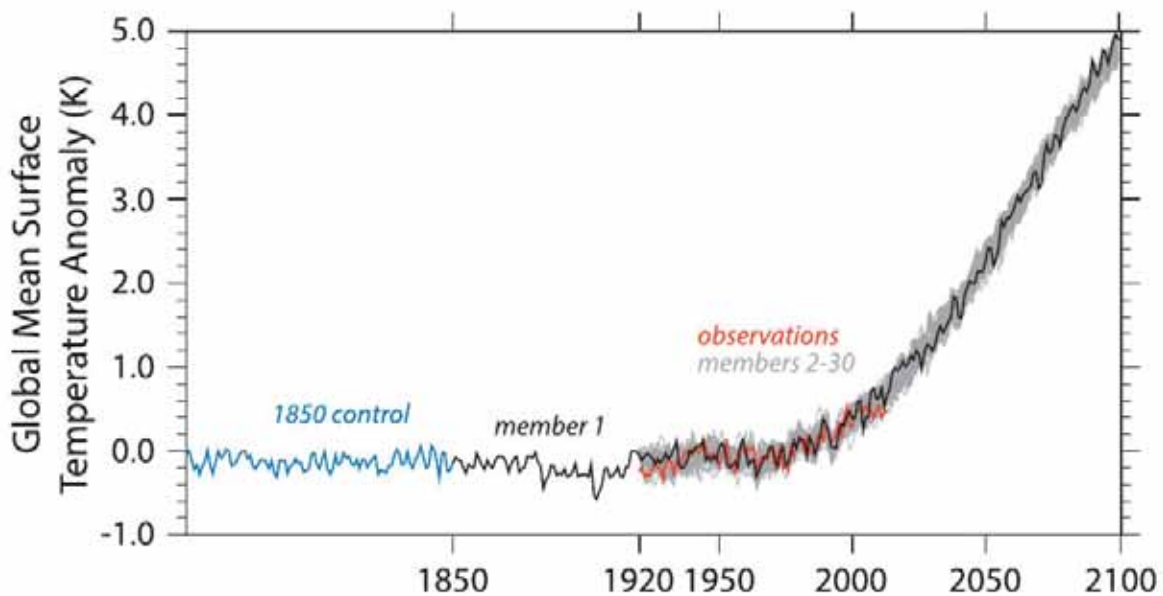
Figure 2.4 – Global surface temperature anomalies (1961-1990 base period) for the PI-control simulation (blue line), individual ensemble members of historical and RCP8.5 simulations (the member one in black line, the other members in grey lines) and observations (red line) from HadCRUT4 (Morice et al., 2012). Reprinted from Kay et al. (2015).
