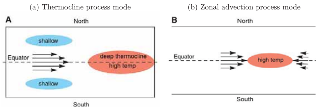
Figure 1.11 – Schematic diagrams of the spatial structure of the two idealized modes resulting from the stability analysis of Fedorov and Philander (2000, 2001). Arrows indicate winds, shaded areas show changes in thermocline depth (“temp” refers to surface temperature). These conditions, during El Niño, correspond to departures from a background state. 1.11a shows the mode associated with the thermocline process, known as the delayed oscillator. 1.11b shows the mode associated with the zonal advection process. Reprinted from Fedorov and Philander (2000).
