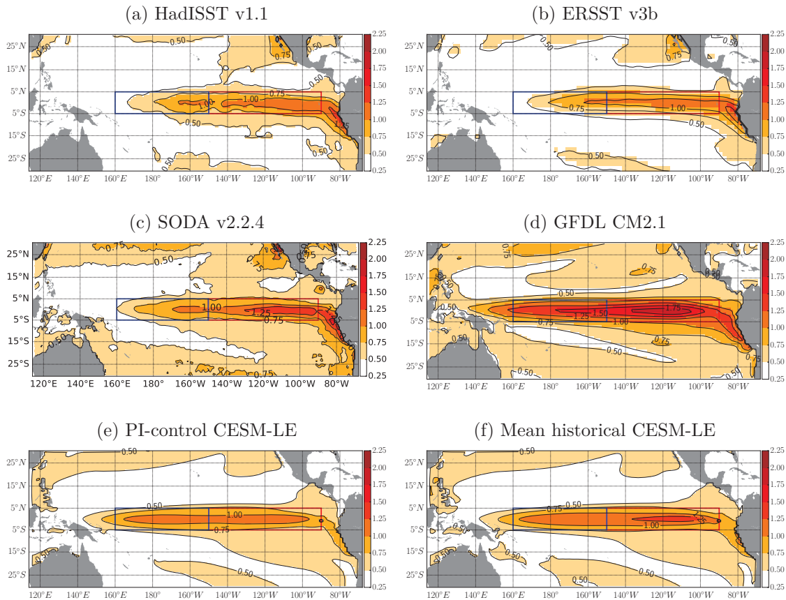
Figure 2.7 – Spatial patterns of the inter-annual SSTA variability (standard deviation) of the tropical Pacific ( 30^\circ\text{S} - 30^\circ\text{N} ) for (2.7a) HadISST v1.1 (1950-2017), (2.7b) ERSST v3b (1950-2017), (2.7c) SODA v2.2.4 (1950-2010), (2.7d) the PI-control simulation of GFDL CM2.1 (500 years), (2.7e) the PI-control simulation of CESM-LE (1801 years) and (2.7f) the ensemble mean of historical simulations of CESM-LE (1 member over 1850-2005 and 41 members over 1920-2005). The boxes represent the Niño-3 (blue) and Niño-4 (red) regions respectively. The data are linearly detrended and the annual cycle is removed.
