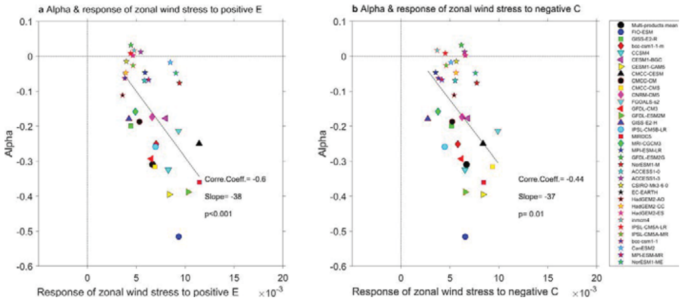
Extended Data Fig. 2 | Inter-model relationship between \alpha and the zonal wind response to SST. a, Relationship between \alpha and the response of monthly zonal wind anomalies to positive E-index values. Zonal wind anomalies are taken at the anomaly centre associated with the E-index.
