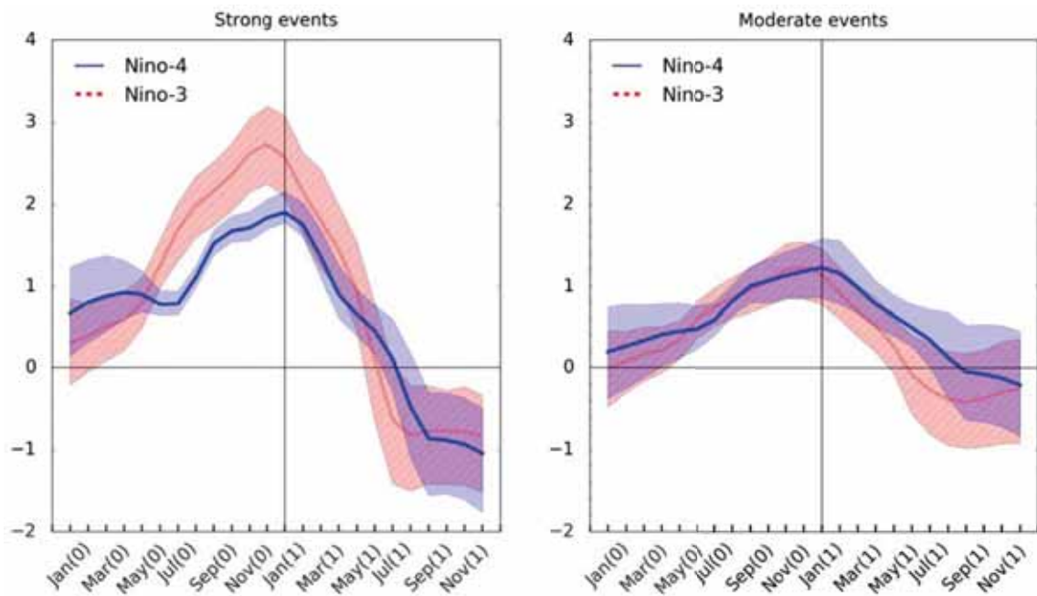
Figure 3.11 – Temporal evolution of CESM-LE historical strong (left) and moderate (right) El Niño events composite for (Fig. 3.11a) the E and C indices and (Fig. 3.11b) the Niño-3 and Niño-4 indices. The shading indicates the range of values between the 25 and 75 percentiles of the distribution of the composite.
