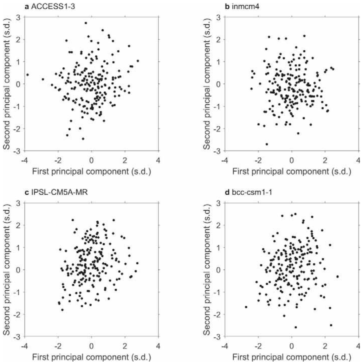
Extended Data Fig. 6 | Examples of the nonlinear relationship between the PC1 and PC2 time series in some non-selected models. a–d, December–February averages for ACCESS1-3 (a), inmcm4 (b),
