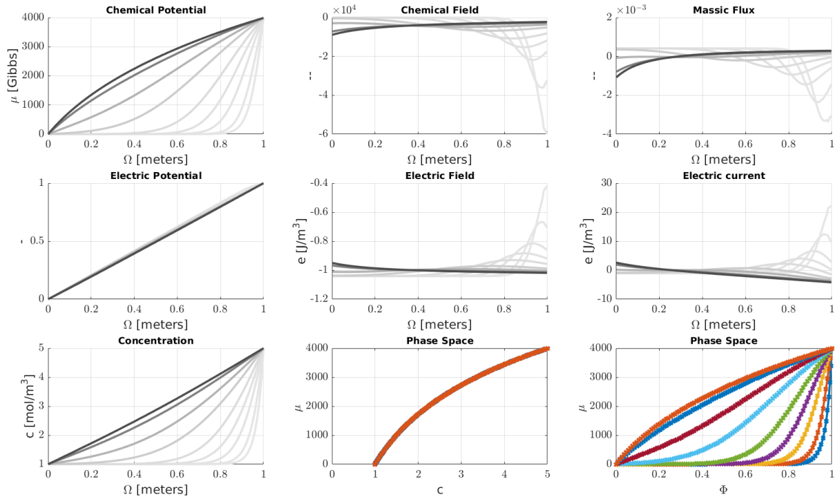
Figure 5.4: Strong bulk coupling, with discontinuity between initial and boundary conditions.
