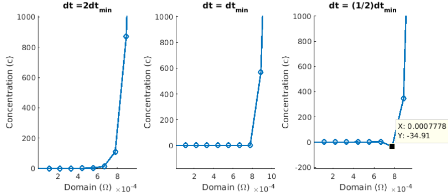
Figure 3.3: Implicit scheme - Spurious oscillation ( \Delta t_{min} )
