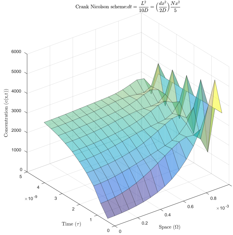
Figure 3.2: Crank-Nicolson scheme - Spurious oscillation ( \Delta t_{max} )
