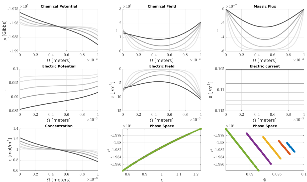
Figure 5.5: Strong bulk coupling using Butler-Volmer BC.
