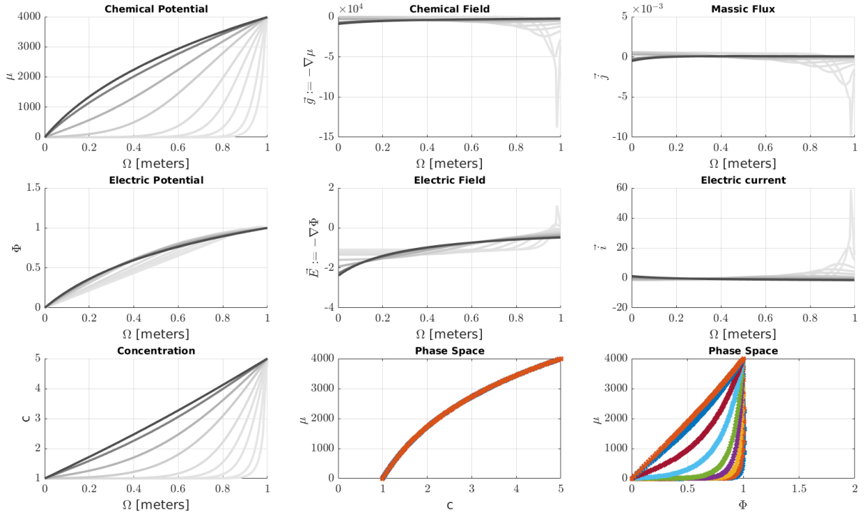
Figure 6.15: Strong bulk coupling with discontinuity between initial and boundary conditions solved using a staggered strategy
