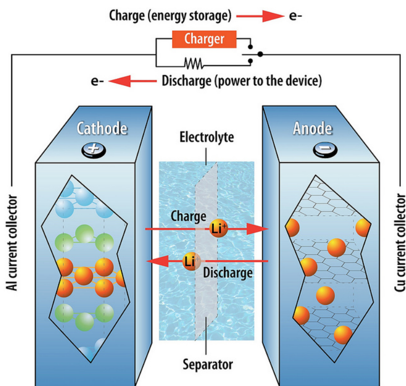
Figure 5.1: How a lithium-ion battery works
