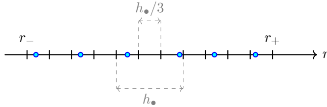
Figure 4.2: A possible choice for the spatial mesh (blue dots are points in \mathcal{L}(u) ).
