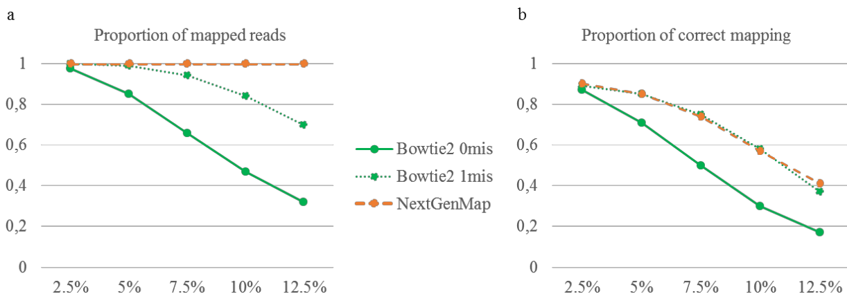
Figure 1: (a) proportion of simulated reads that mapped to the reference, depending on divergence with the reference (b) proportion of correctly mapped reads (amongst all reads).
