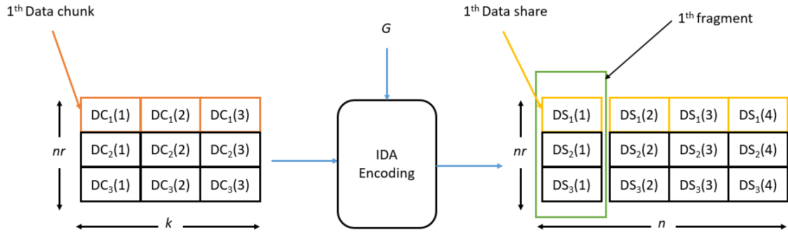
FIGURE 5.8 – Example for k = 3 : Encoding of the i^{th} data chunk DC_i (left) is transformed into i^{th} data share DS_i (right) and i = 1, 2, \dots, nr .
