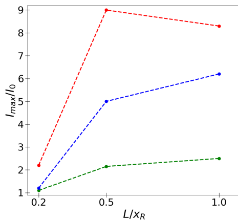
Figure 4.4: Time-averaged beamlet intensity enhancement I_{max}/I_0 as a function of the plasma lengths L/x_R . The green line refers to P^{2D} = 0.5 TW, the blue line refers to P^{2D} = 1 TW, and the red line refers to P^{2D} = 5 TW. Ponderomotive self-focusing in a collisionless plasma.
