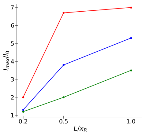
Figure 4.6: Time-averaged beamlet intensity enhancement I_{max}/I_0 as a function of plasma length L/x_R . The green lines refer to P^{2D} = 0.5 TW, the blue lines refer to P^{2D} = 1 TW, and the red lines refer to P^{2D} = 5 TW. Ponderomotive force is activated along with laser absorption.
