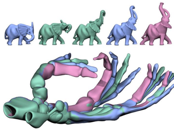
(b) Geodesics in shape space.
