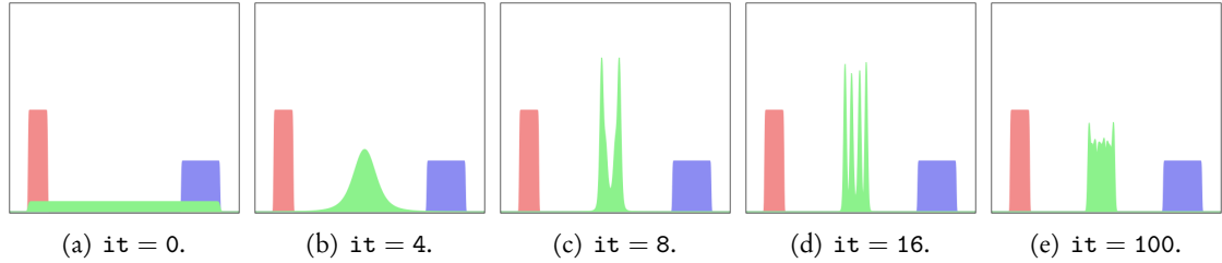
Figure 4.10: Computing a Wasserstein barycenter with a Eulerian scheme, in 1D.
