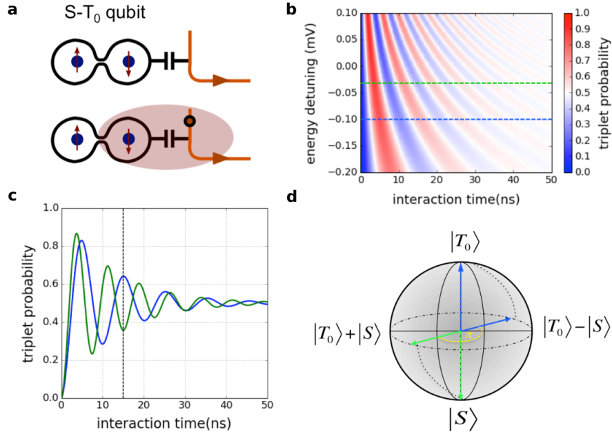
Figure 1.13: Operation of the S- T_0 detector. a , Schematic of a double quantum dot capacitively coupled to an electron waveguide. b , Simulation of the Rabi oscillations, giving the triplet probability as a function of the energy detuning of the quantum dots and the interaction time. c , Triplet probability versus interaction time, for the energy detunings highlighted by the coloured dashed lines in b . d , Bloch sphere representation of the spin-qubit, where a \pi shift is shown between the green and blue arrows, representing the black dashed line in c . The figure is reproduced from [52].
