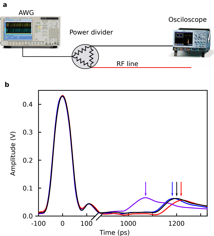
Figure 3.23: Reflectometry set-up. a, Schematic drawing of the reflectometry set-up b, The Gaussians at time equals 0s are the pulses applied in the RF line, while the smaller amplitudes are the reflected pulses. The four arrows indicate the time position of the reflected pulses in the lines connected to the ohmic contact (blue curve), QPC 1 (red curve), QPC 2 (purple curve), QPC 3 (black curve).
