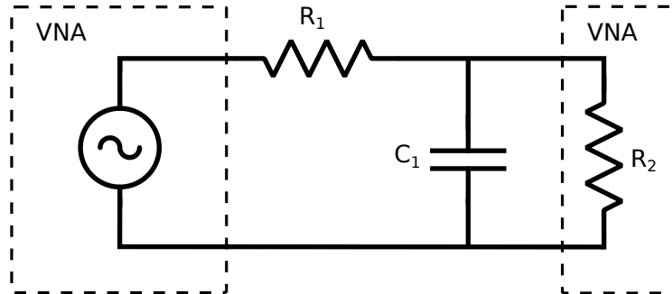
Figure I.1: Electronic circuit using VNA. The VNA is represented by the dashed rectangles, where on the left there is the internal signal generator and on the right R_2 correspond to the 50\ \Omega impedance to ground. R_1 represents the impedance of the Constantan wire together with the resistor of the RC filter. C_1 is the capacitor connected to ground.
