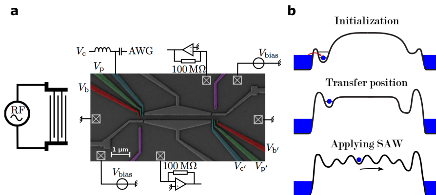
Figure 1.7: Moving quantum dot as a single-electron source. a , SEM image of the sample used as a single-electron transfer device in ref [55]. The two large gates define the 3\ \mu\text{m} -long 1D channel. The purple gates are the QPCs used as an electrometer. Applying a microwave burst to the IDT generates the SAW that will pick up the electron from one QD and transports it to the other QD. b , Sketch of the electrostatic potential during the steps of the transfer protocol. For the initialization, the potential on the QD is lowered to allow one electron to enter. The potential on the QD is then increased to isolate the dot from the reservoir. The applied SAW catches the electron and transports it to the second QD. The figures are adapted from [55, 60].
