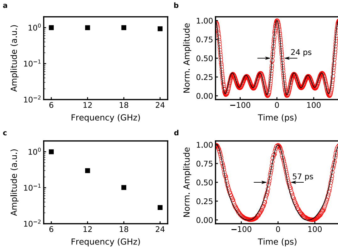
Figure 3.12: Signal generation with the pulse box. a, Amplitude of the 4 different harmonics measured on a sample oscilloscope (WaveExpert 100H) to obtain the minimum FWHM (delta-function-like). The black squares are the amplitudes for the different harmonics. In this case, the values are the same. b, The red dots are the measured signal output on a sampling oscilloscope (WaveExpert 100H) adjusting all the harmonics in phase using the amplitudes from a. The black line is the calculated signal, combining the four harmonics with equal amplitudes. c,d same as c,d but with the difference that the amplitudes of the harmonics decrease exponentially to generate a Lorentzian-like voltage pulse. A 57 ps pulse width is obtained for the best possible Lorentzian (no wiggles in the wings).
