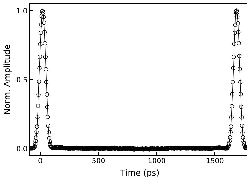
Figure 3.10: Voltage pulse injected at the ohmic contact. Pulse repetition resolved at the sample. The pulses are spaced by 1.66 ns (600 MHz repetition frequency).
