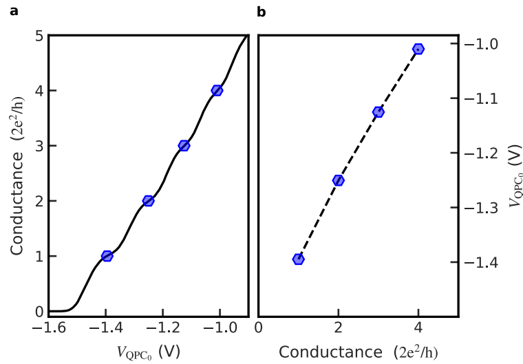
Figure 4.19: Pinch-off of QPC 0 . a , The black line is the conductance versus the applied voltage in the QPC 0 V_{\text{QPC}_0} . The other gates were not polarised. The hexagonal markers correspond to the positions in which the conductance is an integer of 2e^2/h . b , Inversed plot of a . The hexagonal markers are the same as in a . The dashed line is an interpolation of the hexagonal markers. The data was taken with V_{\text{SG}} = 0 V.
