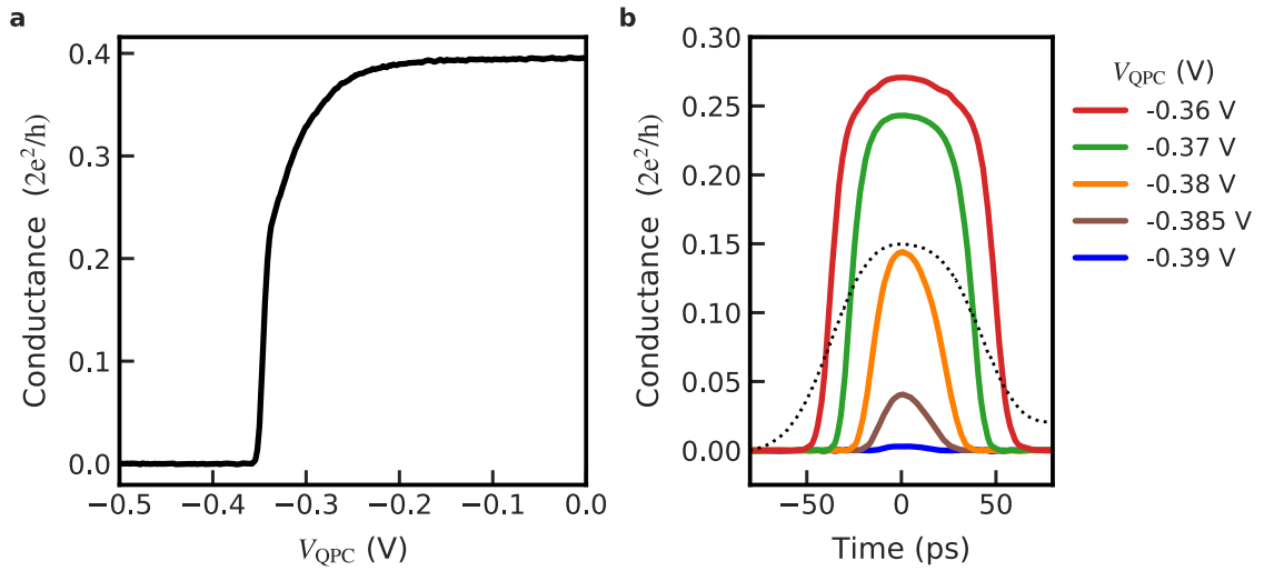
Figure 3.21: Conductance change due to the voltage pulse. a , Conductance of the entire system (ohmic contacts in series with the quasi-1D conductor) as a function of V_{\text{QPC}} b , Expected conductance in the time domain, considering the estimated voltage pulse arriving to the QPC 1 . The different traces correspond to different DC voltage set at the QPC 1 ( V_{\text{QPC}} ). The dashed black line is the voltage pulse at the output of the AWG.
