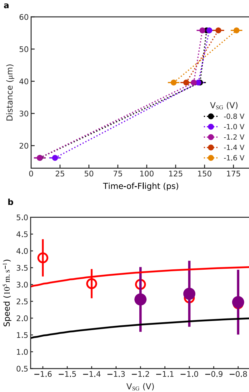
Figure G.2: Time-of-flight and velocity of induced excitation (i). a , Time-of-flight for different confinements V_{\text{SG}} and different distances. b , Velocity as a function of the confinement. The purple circles are the velocity using the QPC as a pump, calculated from a . The red circles correspond to the case in which we use the QPC as a barrier, fixed at the first plateau of conductance. The red curve corresponds to the self-consistent simulations for the plasmon funnelled into a single channel. The black line corresponds to the Fermi velocity, derived from the self-consistent simulations.
