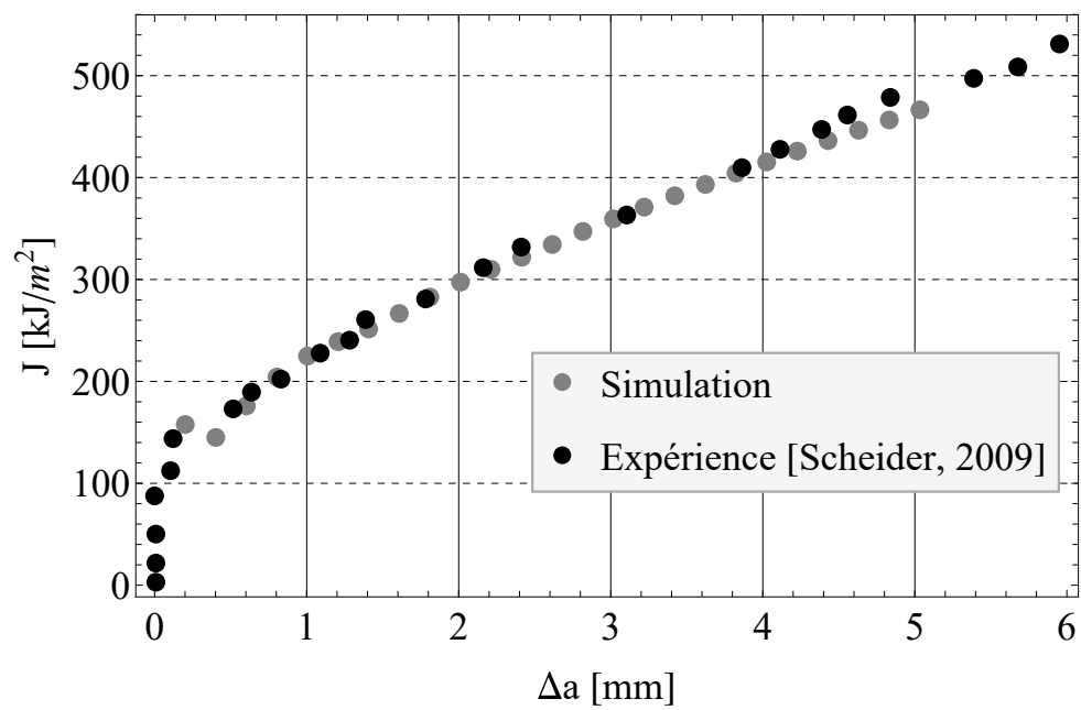
Figure 43 – Courbe de rupture J - \Delta a .
