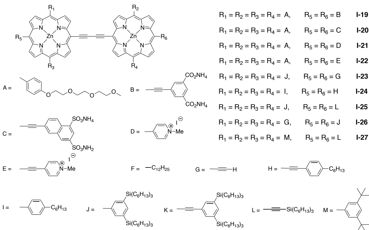
Figure 10. Dimères I-19 à 21, [44] I-22, [44][45] I-23, [46] I-24, [47] I-25, [48] I-26 [49] et I-27 [50]
