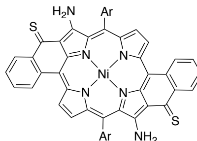
5,15-bis-enaminothioketone
