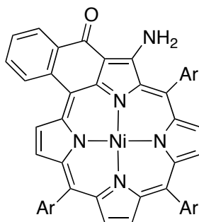
mono-enaminoketone porphyrin
