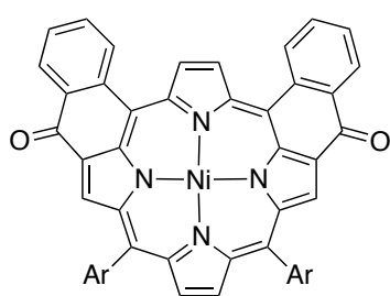
5,10-bi-ketone1-porphyrin
