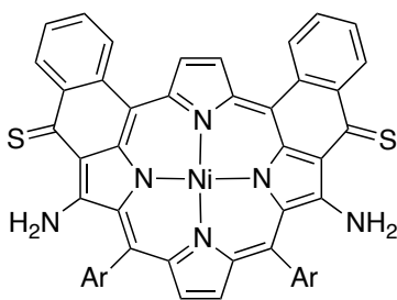
5,10-bis-enaminothioketone
