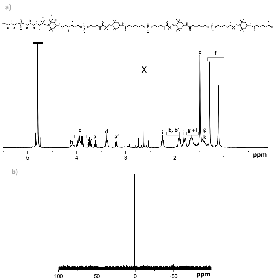
Figure E.5: NMR spectra recorded in D_2O for entry 3 in Table E.1 corresponding to the sequence \alpha\text{-}0aT_30aT_30aT_30aT_3 . a) ^1H NMR, b) ^{31}P -NMR.
