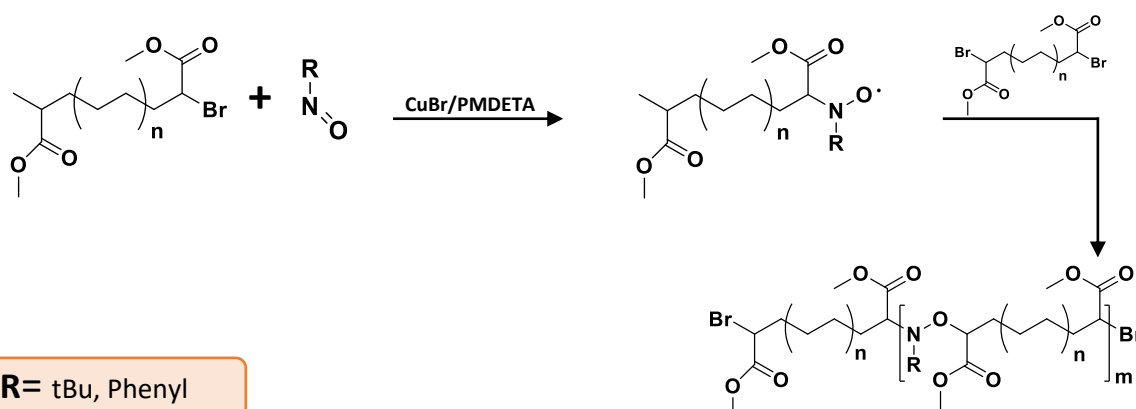
Figure I.8: RACP general strategy for the polymer synthesis.
