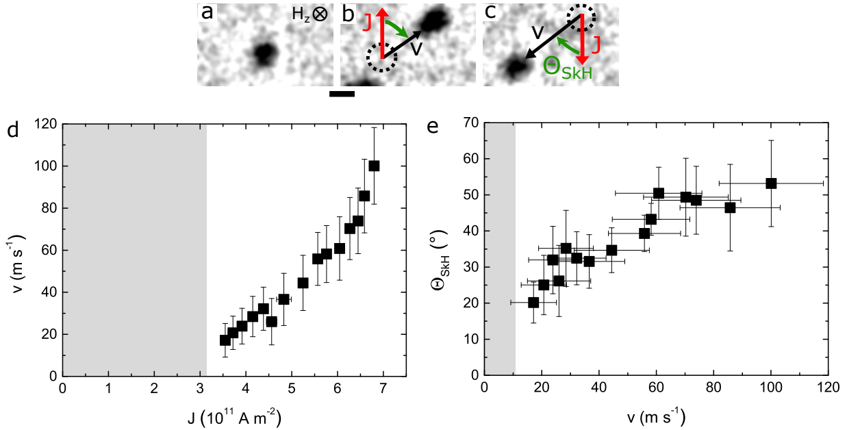
Fig. 5.4: Experimental skyrmion velocity and skyrmion Hall angle | a-c. Sequence of XMCD-PEEM images showing a skyrmion after 2 consecutive 8 ns current pulses with opposite polarities (scale bar is 200 nm). The SkHA, \Theta_{SkH} , is defined as the angle between the current and the skyrmion motion directions. d. Skyrmion velocity as a function of the current density. e. SkHA as a function of the skyrmion velocity. The error bars denote the sum of the systematic measurement error and the standard deviation. The shaded areas highlight the regime for which no significant displacement was observed after injection of a single pulse.
