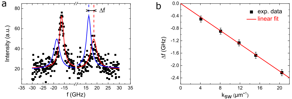
Fig. 5.6: Brillouin light scattering measurements | a. BLS spectrum measured for an IP field \mu_0 H = 0.6 \text{ T} , and for k_{SW} = 20.45 \text{ } \mu\text{m}^{-1} . The black squares are experimental data and the red line is a Lorentzian fit. The blue line is the Lorentzian inverted with respect to f = 0 . \Delta f is the shift between the Stokes and anti-Stokes peak frequencies. b. Frequency shift as a function of the wave vector.
