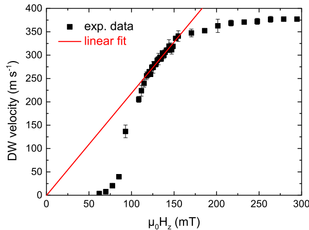
Fig. 5.8: Field-driven DW dynamics experiments | The DW velocity, measured from MOKE microscopy images on a Pt/Co( 0.63\text{nm} )/MgO, as a function of the external OOP magnetic field. The red line is a linear fit in the flow regime.
