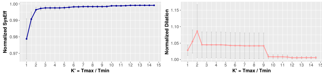
Figure 9.11: Normalized system efficiency and dilation obtained by Algorithm 6 averaged on all 10 sets as a function of K' (with Standard Error bars).
