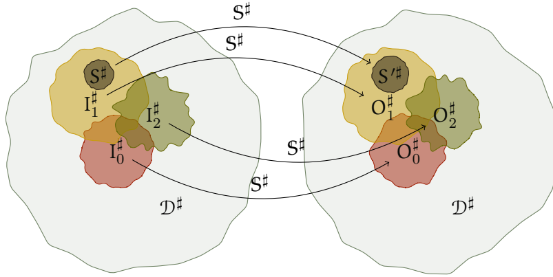
Figure 5.1: \mathbb{T}_2^\# = [I_0^\# \mapsto O_0^\#] \circ [I_1^\# \mapsto O_1^\#] \circ [I_2^\# \mapsto O_2^\#]
