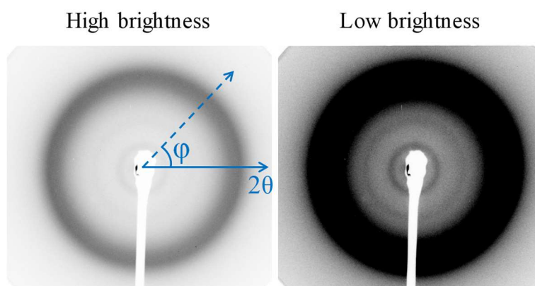
Figure 5-2 – Diffraction pattern obtained on PEBA before stretching, exhibiting a broad outer halo and two inner rings.
