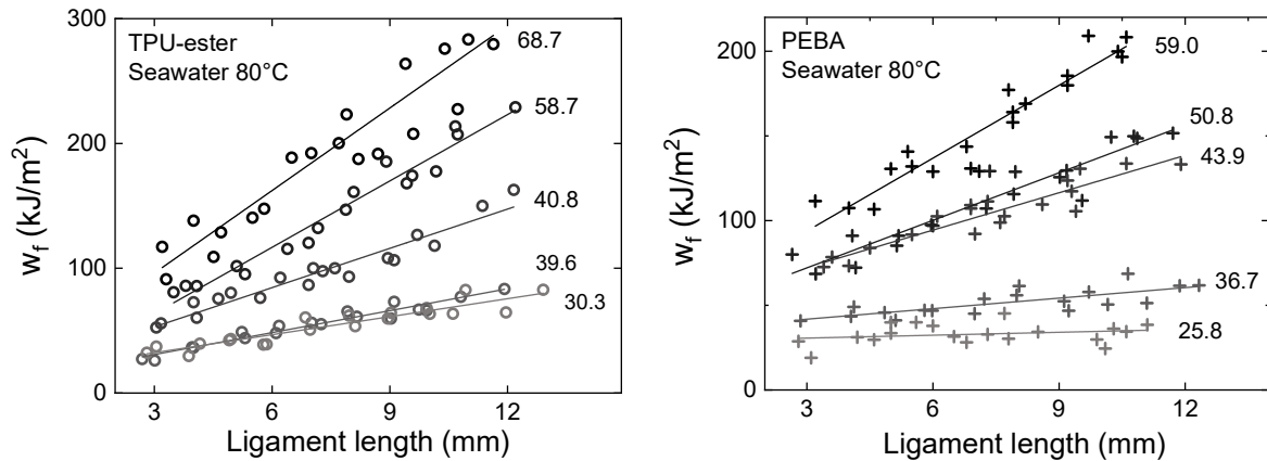
Figure 4-9 – Specific essential work of fracture ( w_f ) as function of ligament length, for TPU-ester and PEBA at different ageing stage (immersion in seawater at 80 °C). Corresponding molar mass ( \text{kg}\cdot\text{mol}^{-1} ) is indicated next to each curve.
