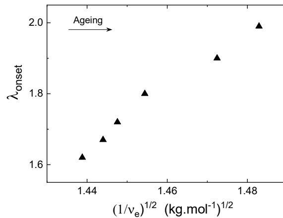
Figure 5-10 – SIC onset relationship with the entanglement network.
