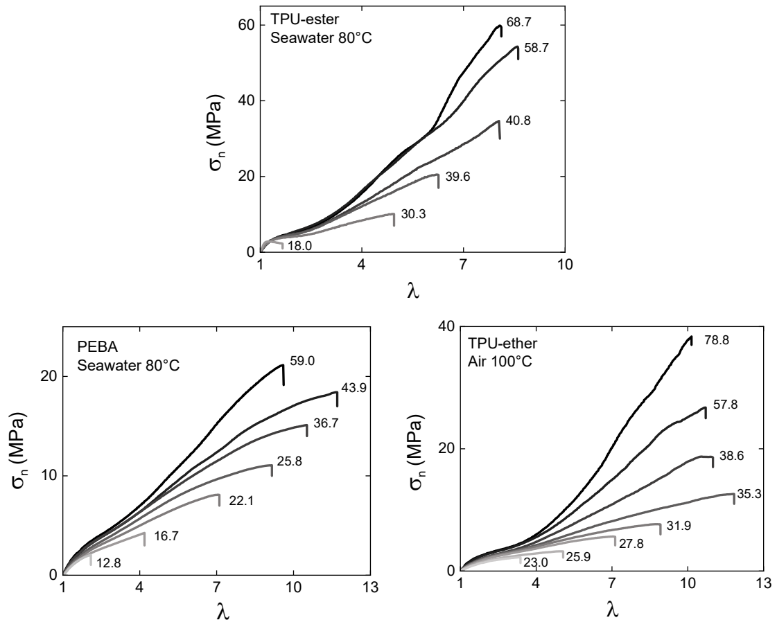
Figure 4-5 – Uniaxial tension behaviour change of TPEs in different exposure conditions. Corresponding molar mass ( \text{kg}\cdot\text{mol}^{-1} ) is reported next to each curve.
