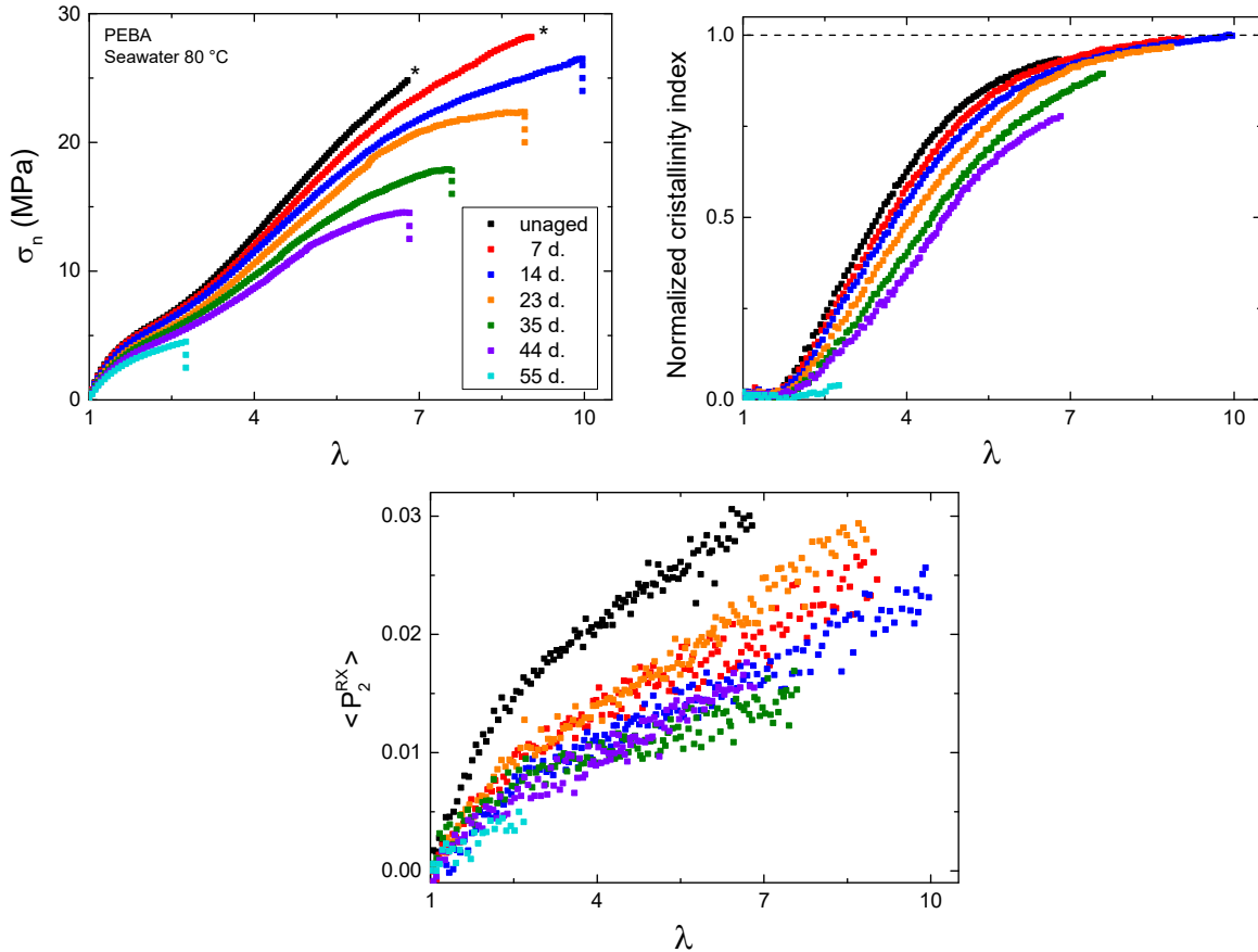
Figure 5-8 – Effect of PEBA ageing in seawater at 80 °C on different parameters.
