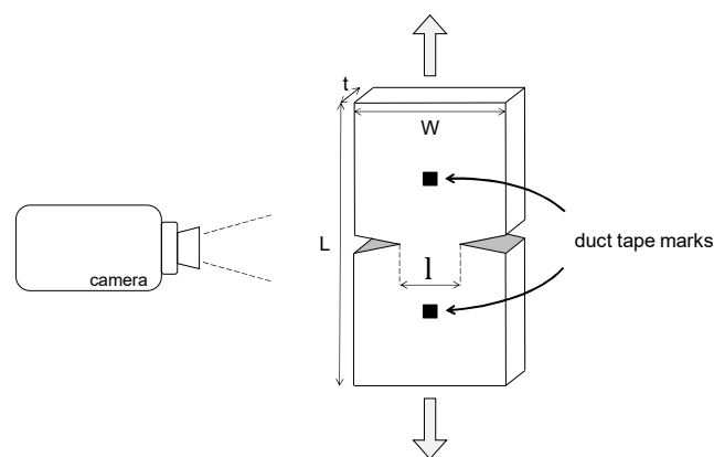
Figure 4-7 - DENT specimen tensile test with an optical extensometer.
