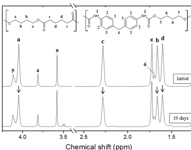
Figure 3-4 - ^1\text{H-NMR} spectra of unstabilized TPU, solubilised in THF, in its initial state and after aging in water at 80 °C for 19 days. Peaks are attributed to corresponding protons with letters for adipate soft block, and numbers for urethane hard block. Peaks identified with an x result from solvent response. Arrows indicate peaks change during ageing.
