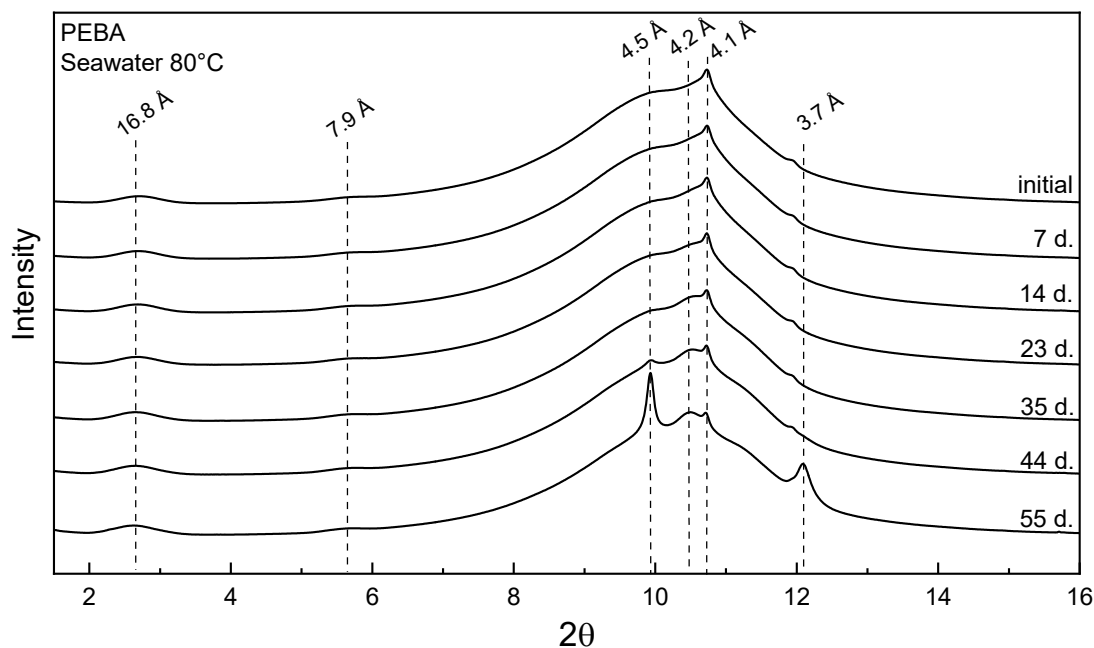
Figure 5-1 – WAXS diffractograms performed in static, on PEBA aged in seawater at 80 °C. Dashed lines represent diffraction peaks positions, with corresponding d spacing.
