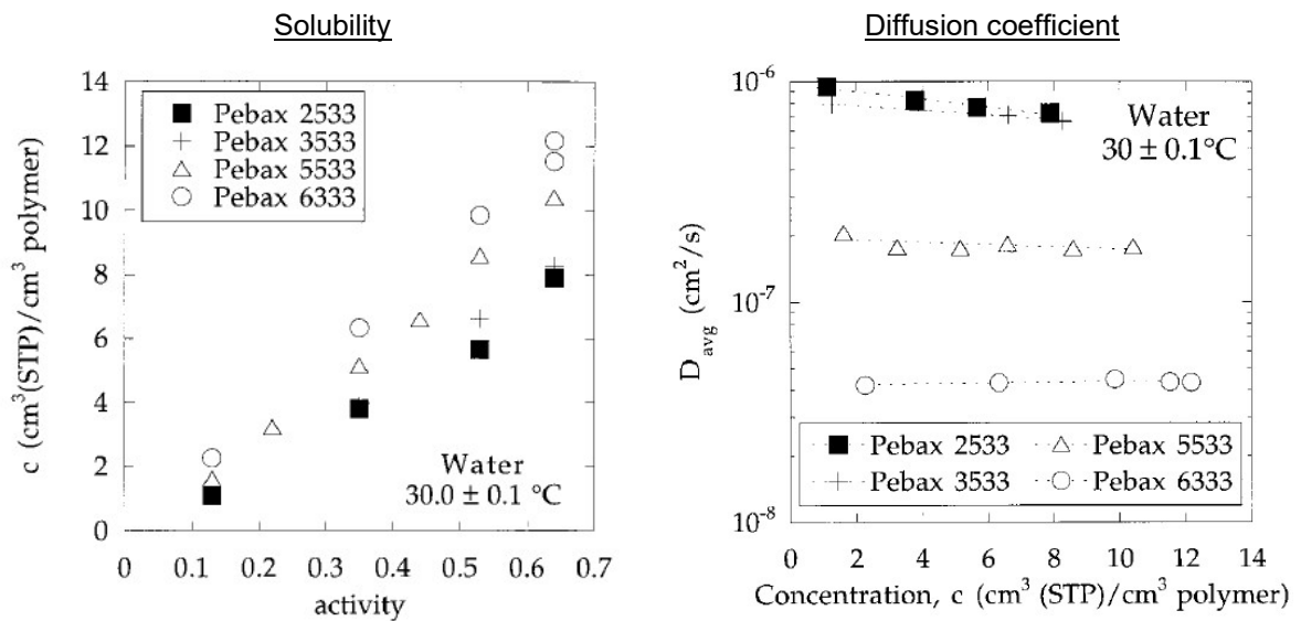
Figure 1-11 - Water solubility vs. water activity and diffusion coefficient vs. water content at saturation for a series of PEBA with various hard block content [63].
