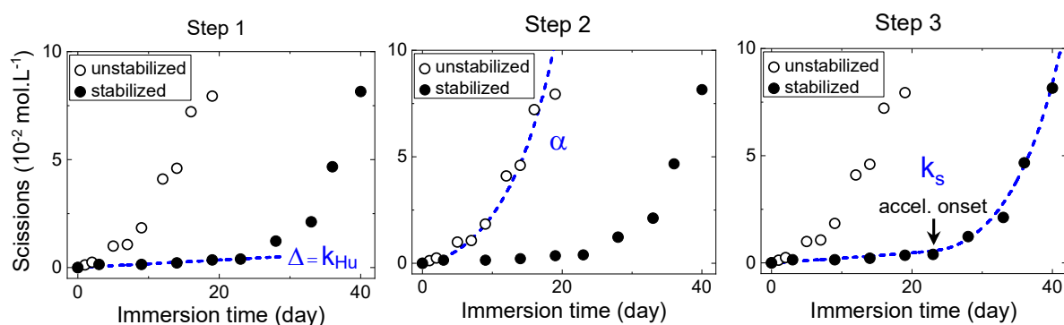
Figure 3-9 - Model constants determination by curve fitting of experimental scissions (ageing at 80 \text{ }^\circ\text{C} ).
