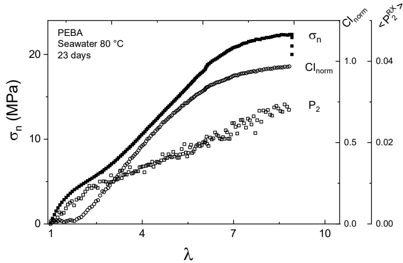
Figure 5-7 – Superposition of nominal stress ( \sigma_n ), normalized crystallinity index ( CI_{\text{norm}} ) and amorphous phase orientation parameter ( \langle P_2^{RX} \rangle ) for PEBA sample aged in seawater at 80 °C for 23 days.
