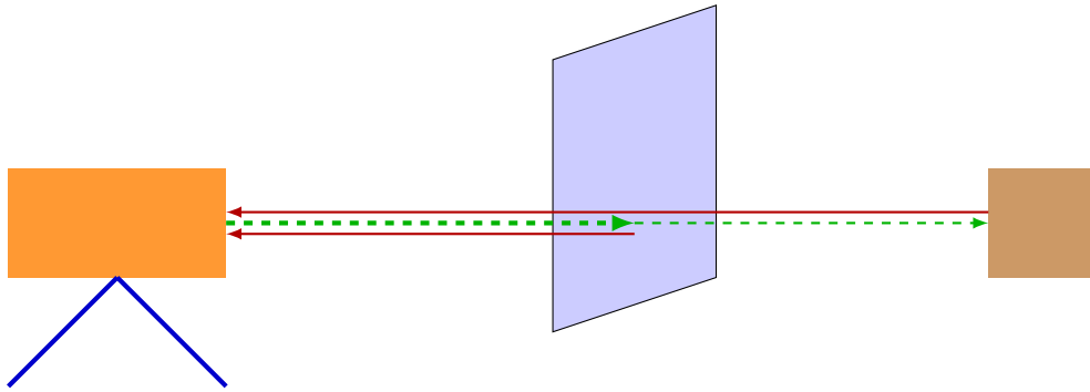
Figure 2.2 – Illustration of the multiple echoes returned for a single light emission. The LiDAR sensor is represented as the orange box, the emitted light in green \rightarrow , the reflected light is in red \rightarrow . First, the emitted light reaches an object that reflects only part of the light: \square . Then, the light that crossed the first object reaches another object: \square , before being reflected in the sensor direction.
