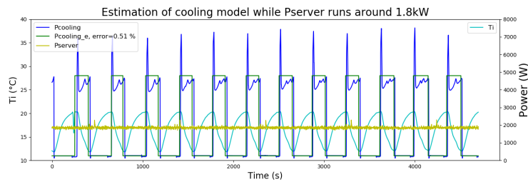
Figure 5.23. Estimation result on training set 2: P_{server} runs around 1.8kW
