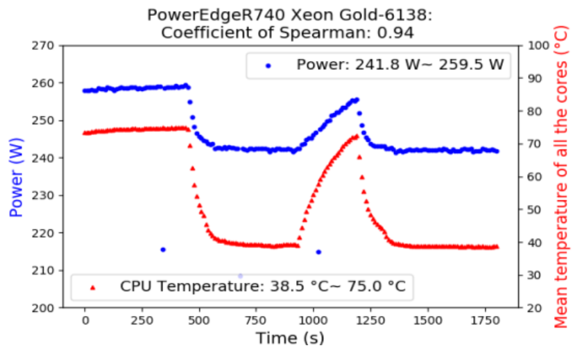
Figure 2.12 – Relationship between CPU Temperature and server power-PowerEdgeR740
