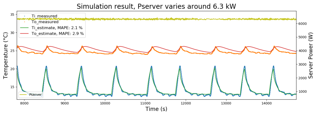
Figure 5.17. Estimation result on training set 3: P_{server} runs around 6.3kW
