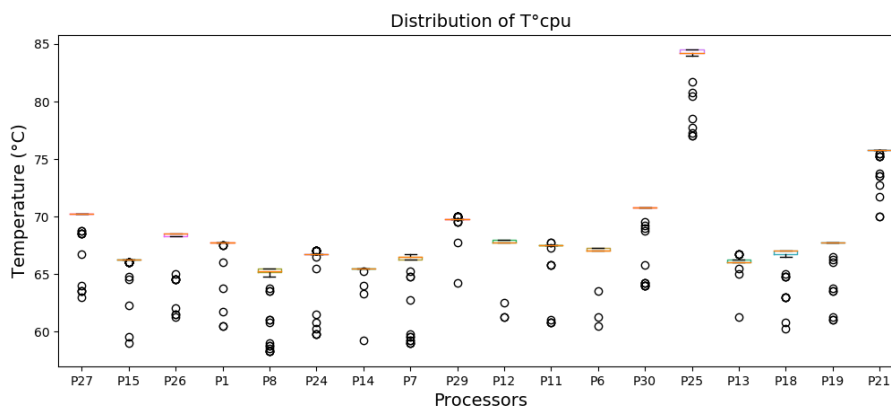
Figure 3.5 – CPU distribution for samples of Xeon E5345
