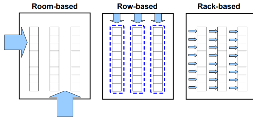
Figure 1.6 – Basic concepts of room, row, and rack based cooling [DR10].
