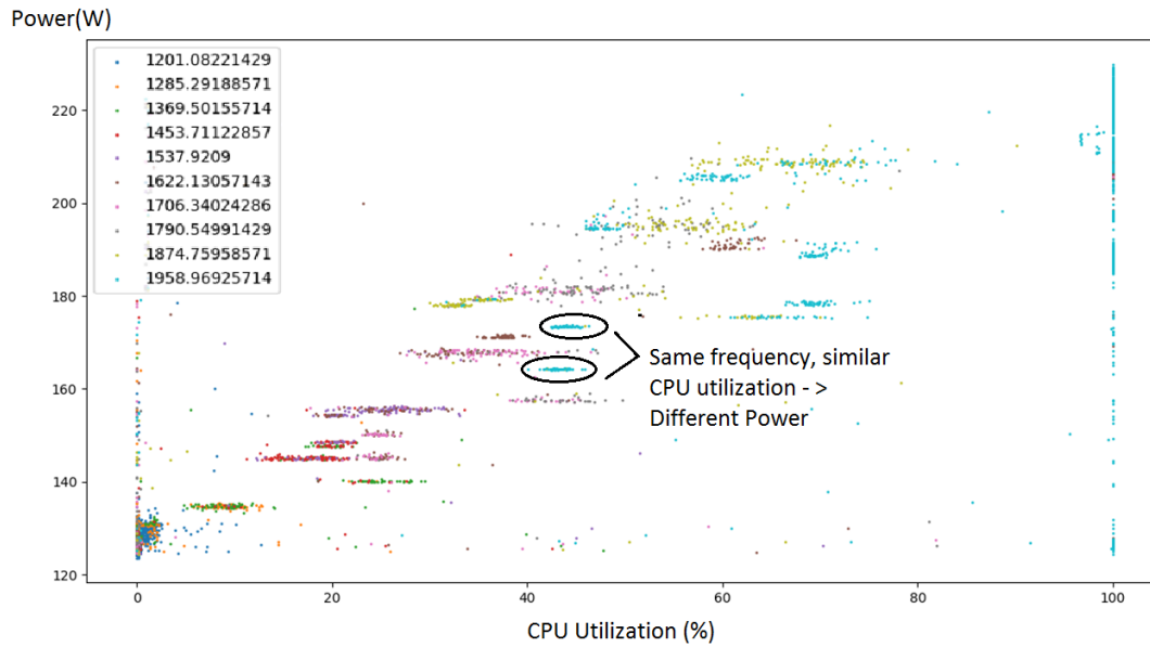
Figure 4.7 – Relationships between CPU-utilization and server power under different frequencies
