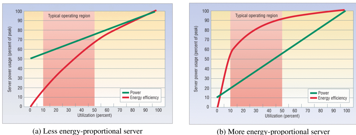
Figure 1.5 – Server power usage and energy efficiency at varying utilization levels [BH07] © 2015 IEEE
