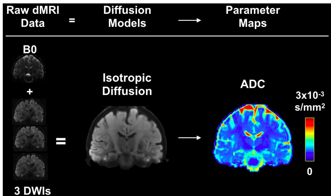
FIGURE 3.3: Isotropic apparent diffusion coefficient model. At least one non-diffusion-weighted (B0) and three DWIs are required for an isotropic diffusion model yielding apparent diffusion coefficient (ADC) maps.
