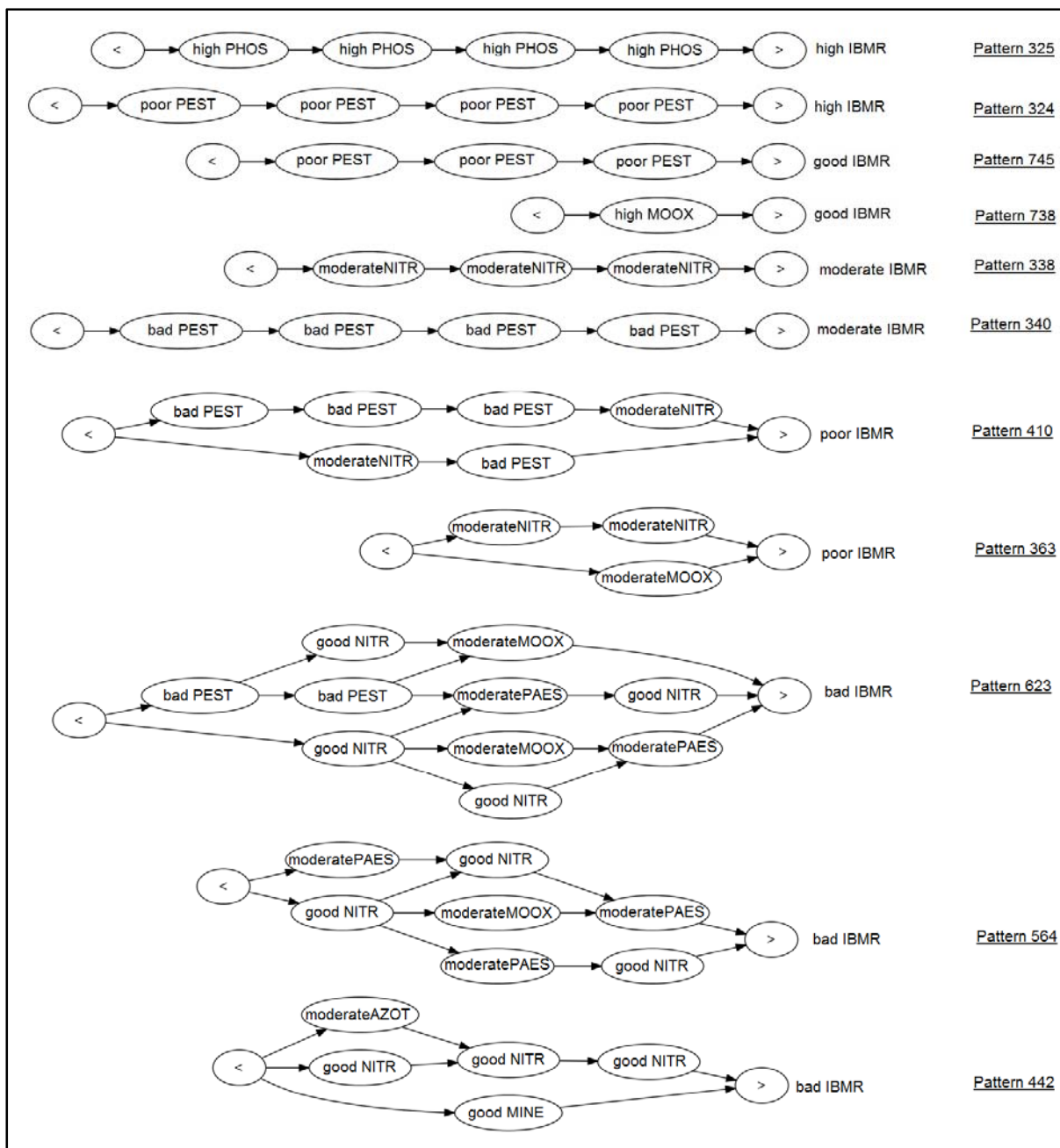
Figure 26: Eleven major patterns extracted from the five contexts of IBMR in the configuration: [area: France, period: 2007-2013, table of thresholds: SEQ, time-length: 24 months, minimum frequency: 0.6]
