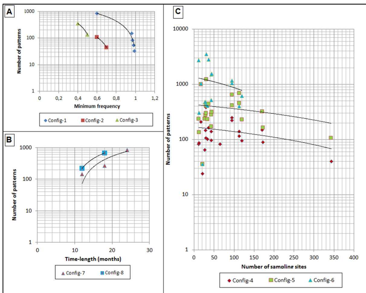
Figure 21: Variation in the number of patterns according to: A: variation in minimum frequency, B: variation in time-length, C: variation in the number of sampling sites; extractions obtained with 8 configurations for period: 2007-2013: Config-1& 3 = [area: France, table of thresholds: SEQ, min. frequency: VARIABLE, Config-1, time-length: 24 months, Config-3, time-length: 6 months]; Config-2= [area: Paris and surroundings, table of thresholds: SEQ, time-length: 6 months, min. frequency: VARIABLE]; Config-4 & 5 = [area: VARIABLE, table of thresholds: SEQ, time-length: 12 months, Config-4 min. frequency: 0.8; Config-5 min. frequency: 0.6]; Config-6 = [area: VARIABLE, table of thresholds: WFD guide, min. frequency: 0.6]; Config-7 & 8= [area: France, time-length: VARIABLE, Config-7 table of thresholds: SEQ min. frequency: 0.6], Config-8 table of thresholds: WFD guide, min. frequency: 0.8]
