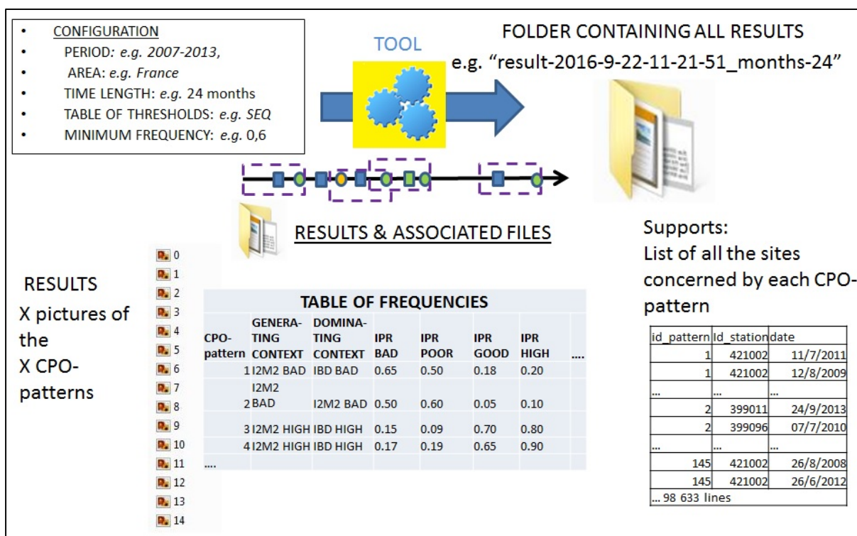
Figure 20: Diagram of the results and the associated files generated by PRESTOR when extracting patterns
