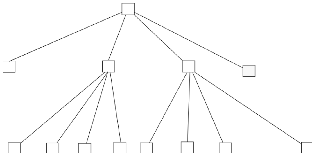
FIGURE 5.1 – Un quadtree.
