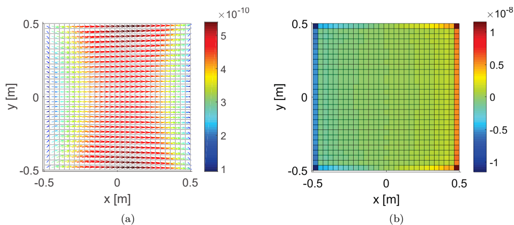
Figure 4.3: a ) Electric polarization (real part) distribution, ( \text{C/m}^2 ). b ) Electric charge density distribution ( \text{C/m}^3 ).
