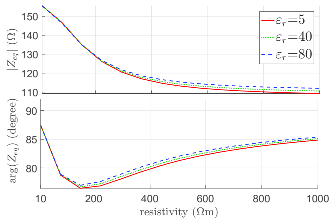
Figure 5.15: Z_{eq} of the embedded coil for a concrete resistivity from 10 \Omega\text{m} to 1000 \Omega\text{m} , parametrized for \epsilon_{rc} equal to 5, 40, and 80.
