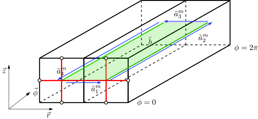
Figure B.3: Algebraic relations between \tilde{\mathbf{b}} and \tilde{\mathbf{a}}^m for the Cell Method approach.
