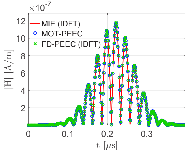
Figure 6.4: Scattered magnetic field norm for case 1).
