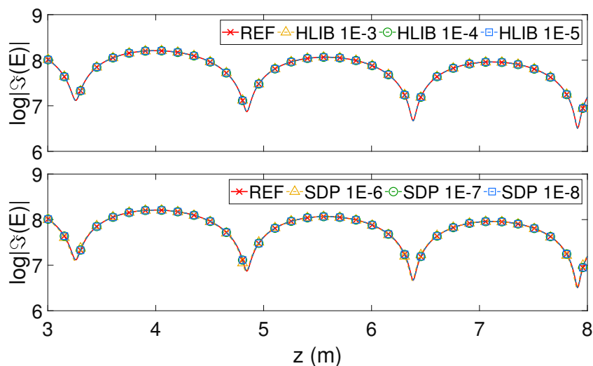
Figure 5.7: \log|\mathfrak{S}(\mathbf{E})| along a line (top: HLIBPro, bottom: SDP)
