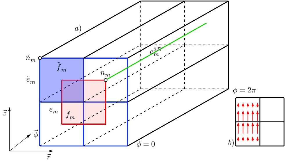
Figure B.4: a. Primal and dual geometric entities for the magnetic grid of the Coulombian axisymmetric formulation. b. Axial symmetric w^{rz} edge shape function.
