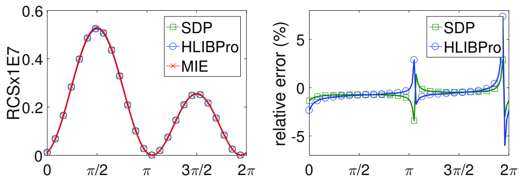
Figure 5.5: RCS along a yz -circular target, distance 500 m.
