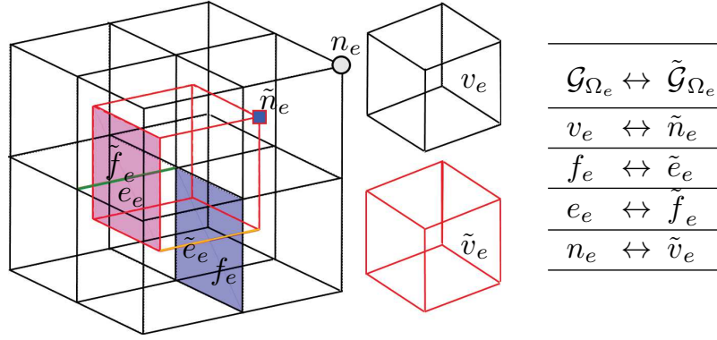
Figure 3.2: Primal and dual grids for the case of a hexahedral structured mesh.
