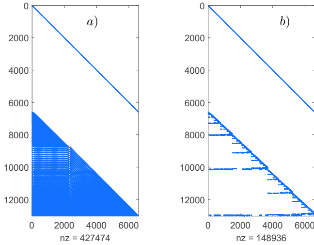
Figure 4.1: \text{RREF}(\mathbf{D}_{\Omega_e}^*)^T obtained without (a) and with (b) the reordering technique.
