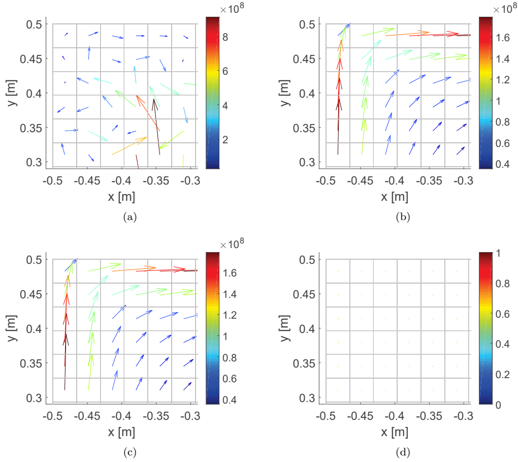
Figure 4.2: Current density (real part) distribution obtained from: a) the direct solution of (4.16), b) the loop–star change of basis strategy, c) the loop change of basis strategy, and d) the star change of basis strategy. Values in \text{A/mm}^{-2} .
