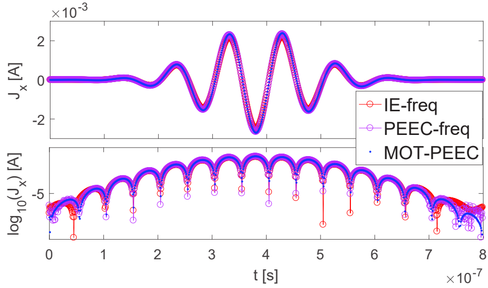
Figure 6.10: Current evolution on the square plate excited by a GMP.
