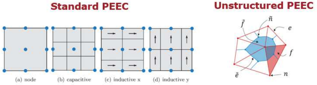
Figure 1.8: PEEC method, standard discretization vs unstructured discretization. 2-D model.
