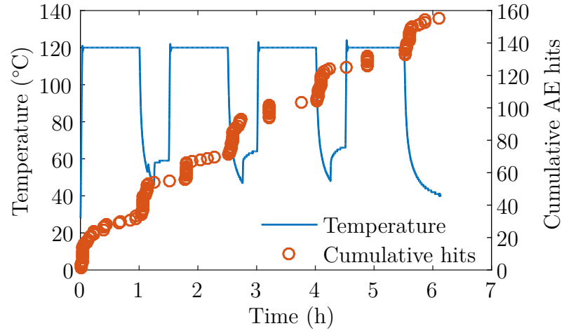
Figure 6.2 Variation of the temperature and the cumulative AE hits as a function of time during the temperature cycling test of an AP 5HS C/PPS. Most of AE hits occur during the first temperature increase or during temperature decreases. AE hits from the first temperature increase may be damage-related ( e.g. , process-based defects), however AE hits from unloading should be noise-related ( e.g. , friction-based). Therefore, temperature cycling seems to result in insignificant damage development. However, it may induce additional AE signals.
