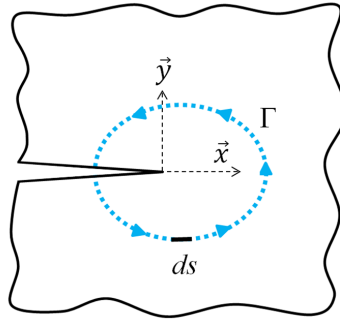
Figure 2.27 Illustration of the J contour integral.
