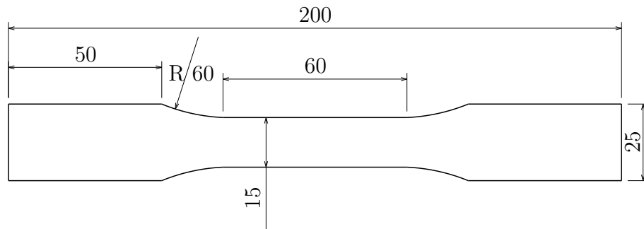
Figure 4.4 Specimen geometry. The dogbone specimens were waterjet-cut from plates. The specimen length, width and thickness were around 200, 15 and 2.3 mm, respectively.
