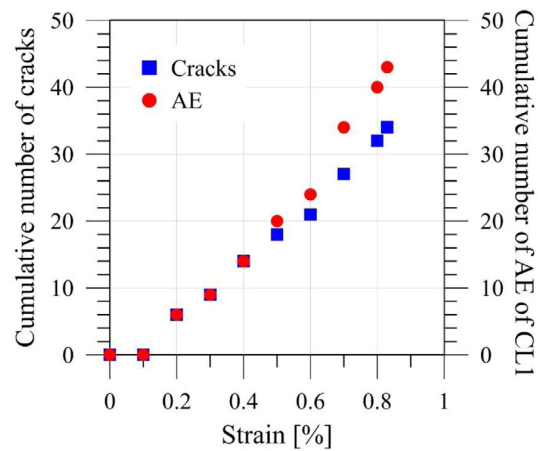
Figure 2.18 Comparison of the cumulative AE events associated with intra-bundle cracking (cluster 1) and the cumulative number of intra-bundle cracks as a function of strain in a 5 mm central portion within 5HS C/PPS laminates at RT [62]. The AE events were obtained after a k-means++ algorithm, whereas the number of intra-bundle cracks were monitored through edge observations. A very good correlation can be observed between AE events and intra-bundle cracks.
