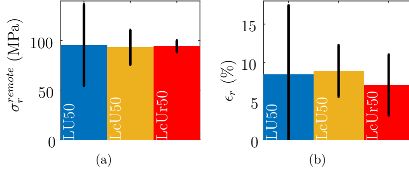
Figure 5.8 (a) Remote stress and (b) strain at failure of AP SEN specimens subjected to various test conditions at 120 °C (the error bars represent the 95% confidence interval). This figure suggests that the ultimate failure is not influenced by time-dependent phenomena.
