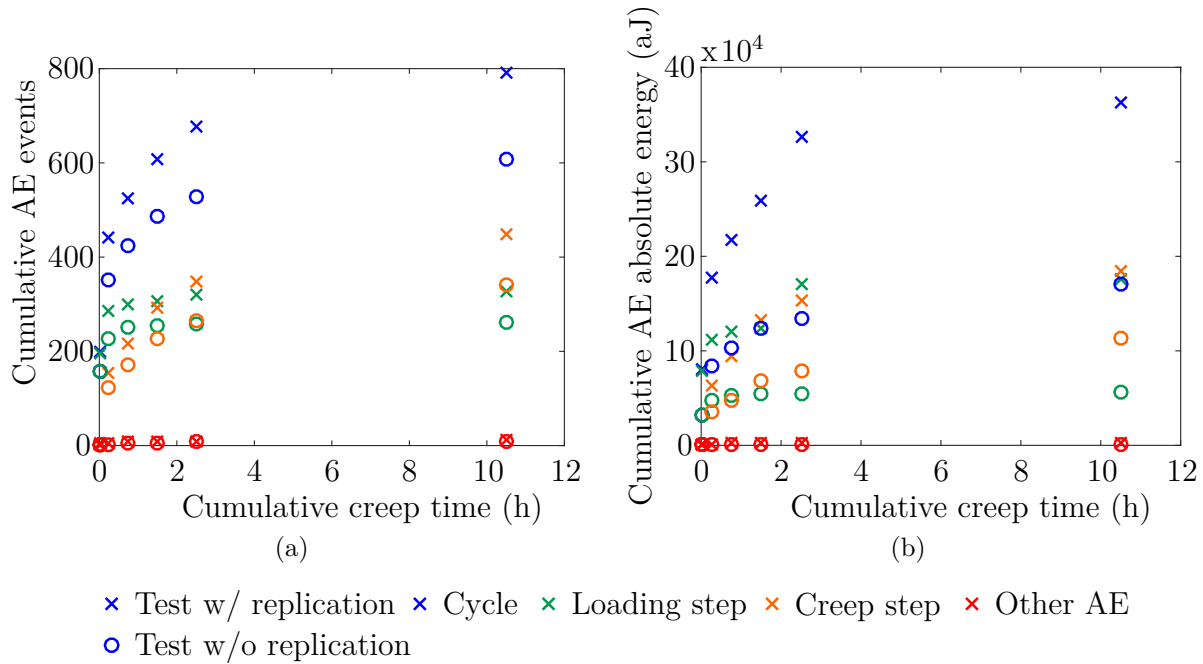
Figure 6.20 AE activity per cycle within a 15 mm centered region during 60 MPa CC tests on AP 5HS C/PPS at 120°C: (a) cumulative events and (b) cumulative absolute energy. The AE activity increase during creep steps may reflect time-dependent damage. The AE activity during unloading and recovery stages is insignificant. Creep steps induce less AE activity than loading phases in terms of quantity and energy.
