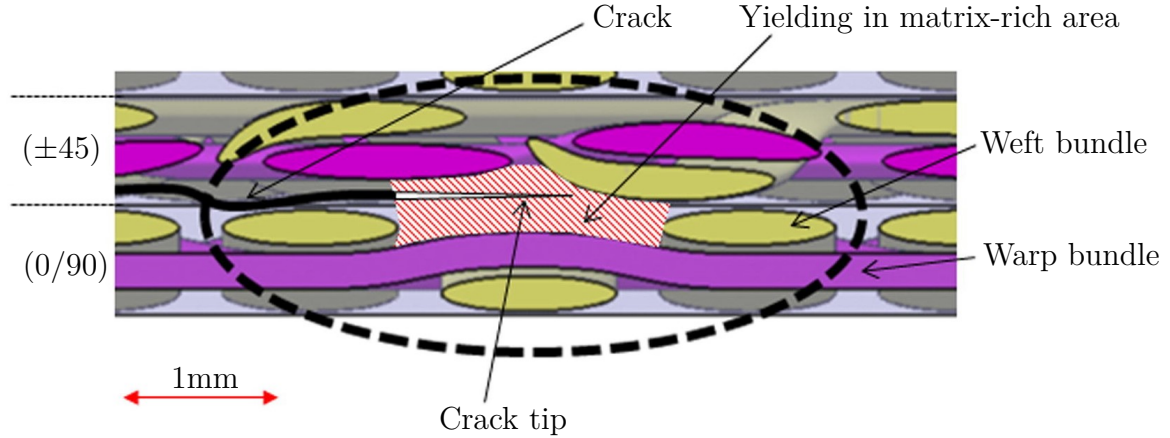
Figure 1.1 Illustration of the propagation of an inter-laminar crack within the mesostructure of a QI woven-ply laminate and possible interaction with a resin-rich area. Only two plies are represented: one (0/90) ply and one ( \pm 45 ) ply. The mesostructure of woven-ply laminates displays resin-rich regions that may delay damage propagation through crack blunting depending on the matrix' mechanical behaviour [6, 7].
