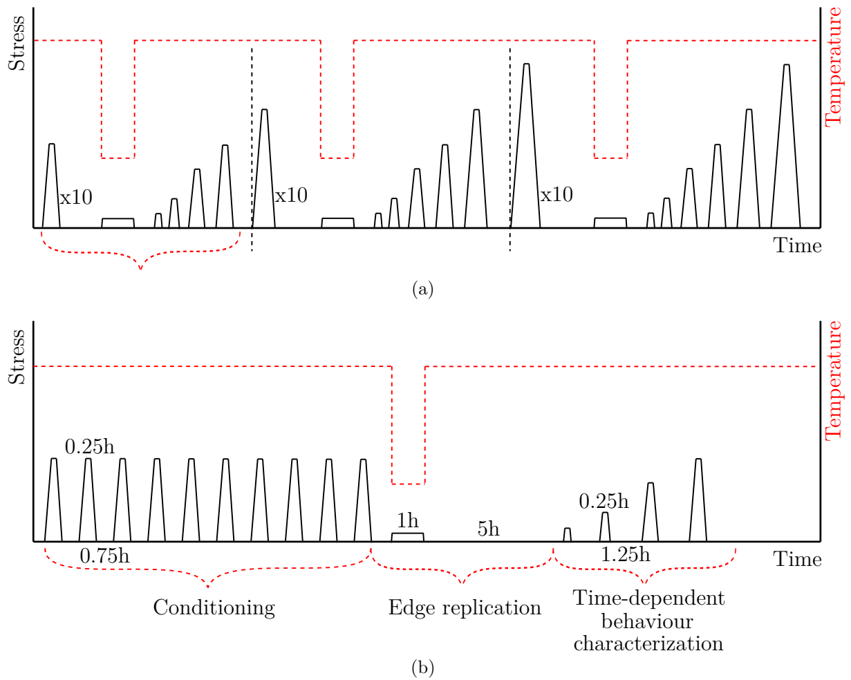
Figure 7.1 (a) Protocol of the damage effect study on the macroscopic viscoelastic behaviour (based on [69]) with three damage states. (b) Zoom on one damage state of the previous protocol.
