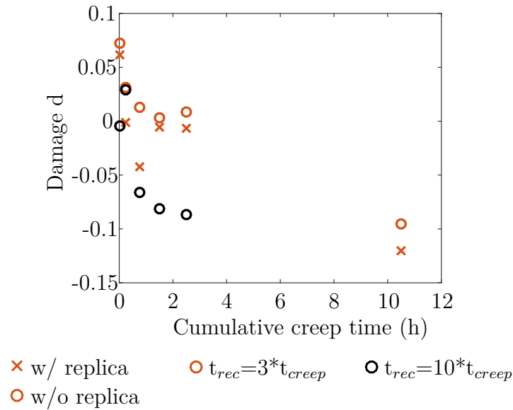
Figure 6.25 Damage variable d as a function of cumulative creep time for several CC tests on AP 5HS C/PPS at 60 MPa and 120 °C. Unrecovered viscoelasticity is not at the origin of the decrease in d . A faster decrease is observed during the test with higher recovery times. It suggest that the decrease results from some thermal aging effect.
