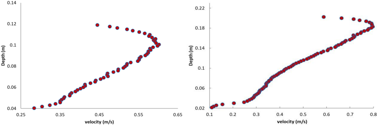
Figure 3.3- Horizontal Velocity Profile (second sensor) at the first measuring site 1.5cm from the outer wall (10cm depth of flow)
