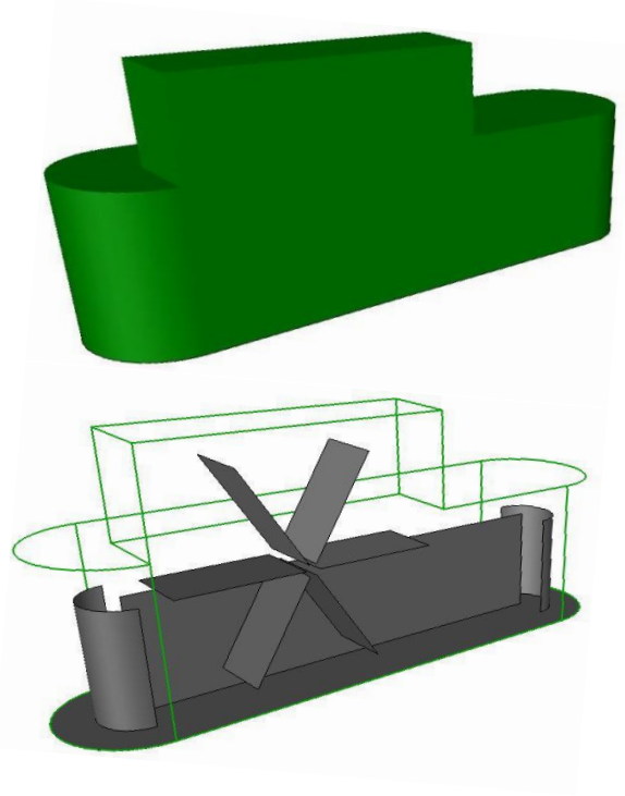
Figure 2.11- Geometry of HRAP (up) and layout with baffles, middle wall and paddlewheel (bottom) for Dynamic Mesh Method using SALOME
