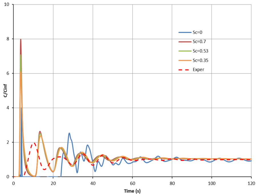
Figure 4.18 - Impact of turbulent Schmidt number on virtual tracer experiment ( U_{average} = 0.311 m/s, 20 cm depth)
