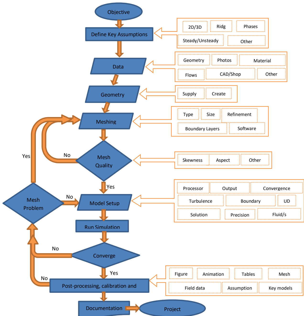
Figure 2.8- Complete Flow CFD modelling processes. Source (Wicklein et al., 2016)
