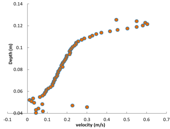
Figure 3.23- Average Vertical Velocity Profile at the first measuring site (Average of the three measuring points) (10cm depth of flow)
