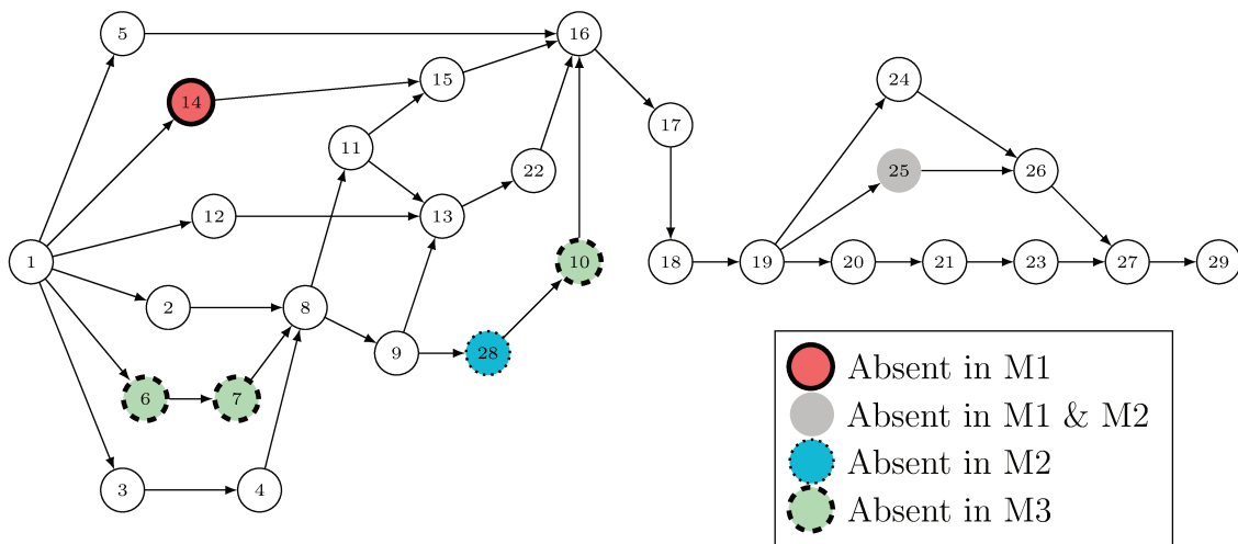
Figure 5.2: Combined precedence diagram of agricultural mulchers (Maccini, 2017)
