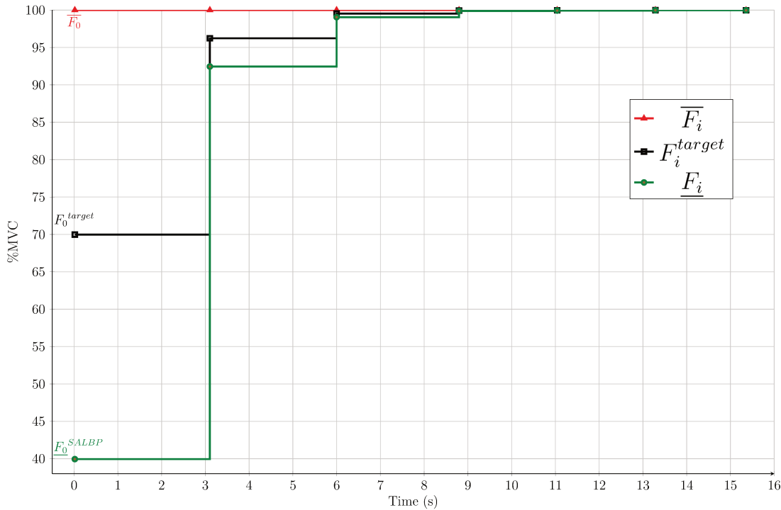
Figure 5.3: The evolution of bounds in the execution of IDS with the solution of SALBP-1 as starting solution - agricultural mulcher assembly line
