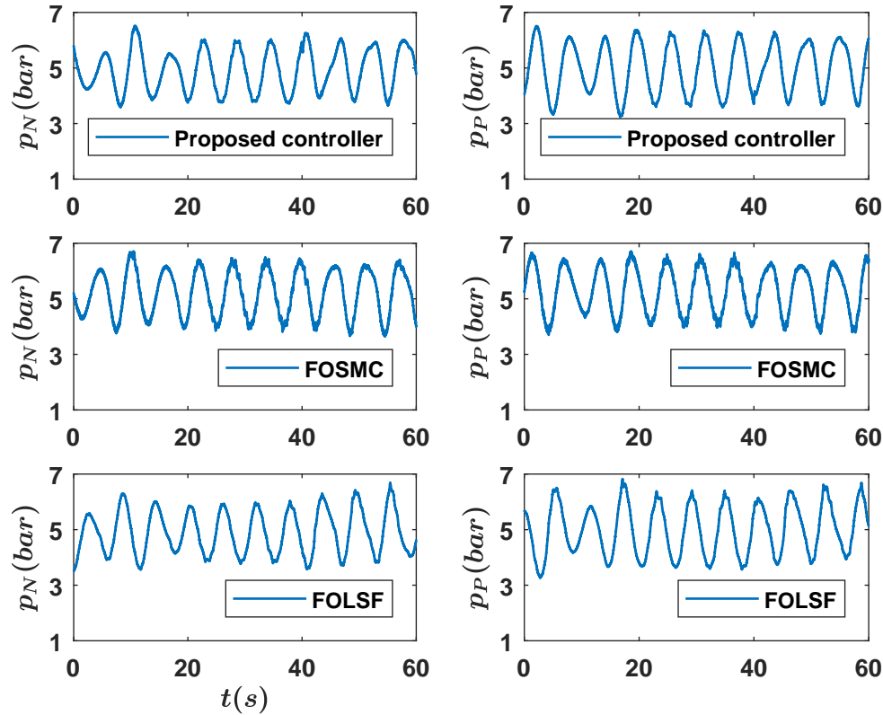
Figure 5.7 – Left pressure p_N(\text{bar}) versus time ( s ) Right pressure p_P(\text{bar}) versus time ( s ) for controller (2.15)-(2.16) ( Top ), FOSMC ( Middle ) and FOLSIF ( Bottom ).
