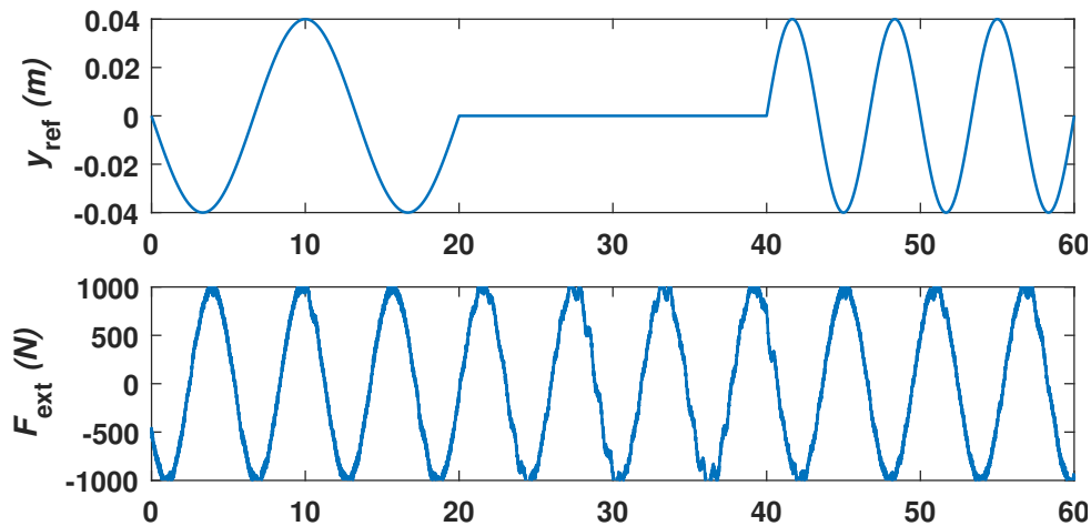
Figure 5.3 – Top. Reference trajectory y_{\text{ref}} \text{ (m)} for the actuator position versus time (s). Bottom. External perturbation F_{\text{ext}} \text{ (N)} versus time (s).
