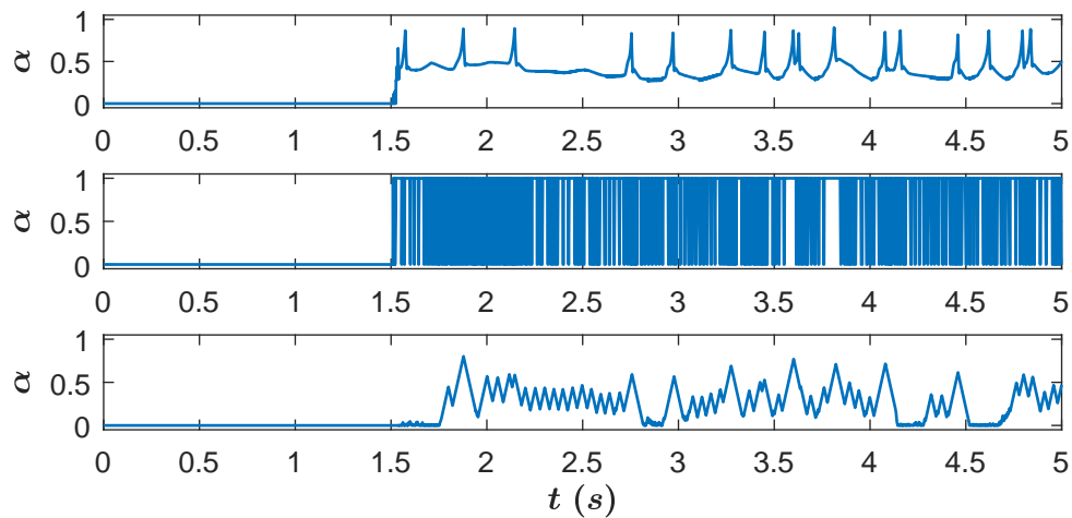
Figure 3.7 – Evolution of \alpha versus time ( s ). Top to bottom: controller with algebraic- \alpha approach ( Set1 ), controller with switching- \alpha approach ( Set1 ), controller with dynamic- \alpha approach ( Set1 ).
