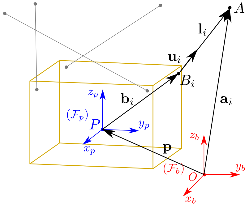
Figure 2.2: CDPR geometric parametrization.
