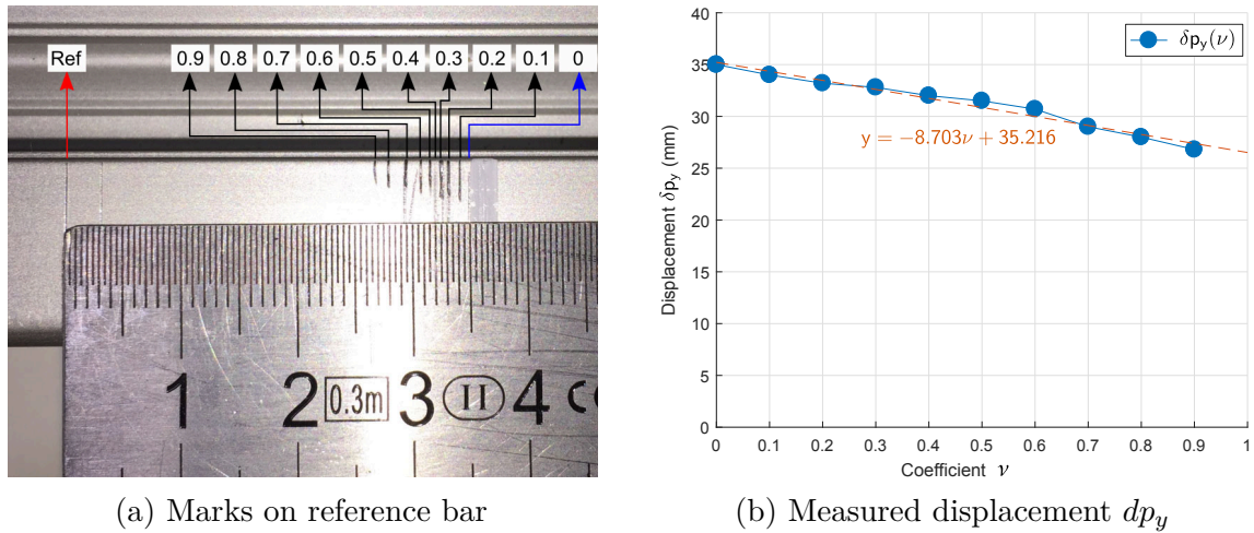
Figure 4.42: Measured platform displacement \delta p_y under a 50 N force along y_b axis depending on value of \nu .
