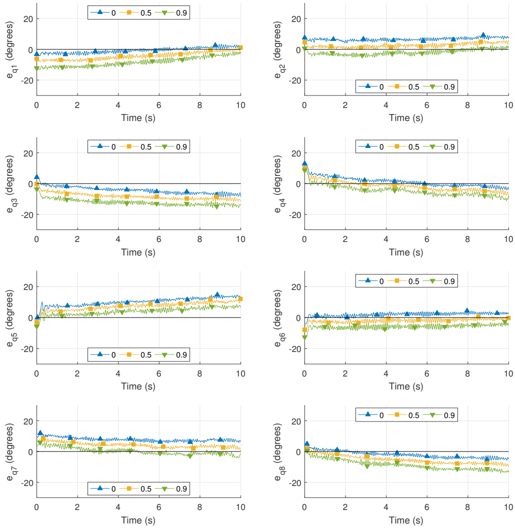
Figure 4.46: Motor position errors e_q as a function of coefficient \nu .
