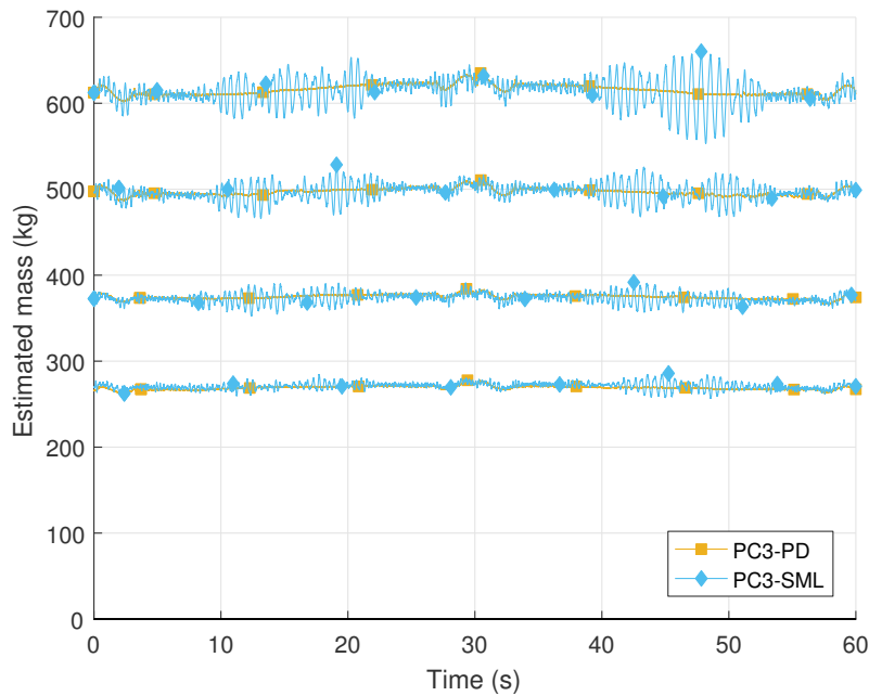
Figure 4.24: Estimated mass (kg) for the four payloads with PC3-PD and PC3-SML control schemes along trajectory.
