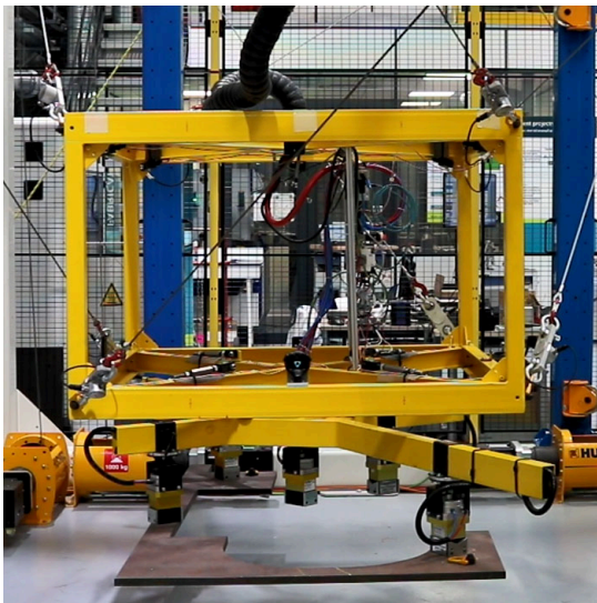
(c) Platform with plate M1 (MPM1, 488 kg)
