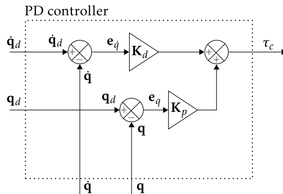
Figure 4.10: Internal structure of the PD controller.
