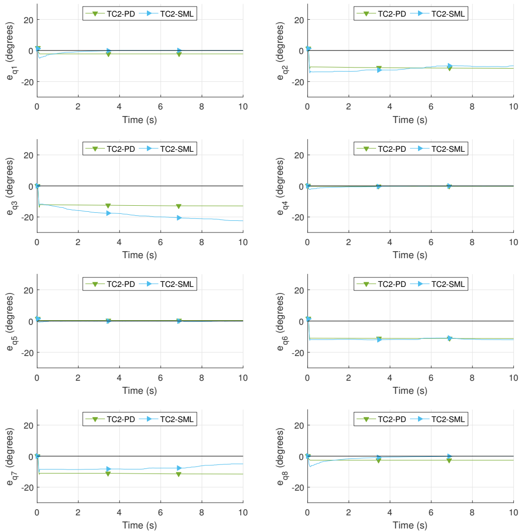
Figure C.1: Motor position errors \mathbf{e}_q for PD and SML controllers with TC2 control architecture
