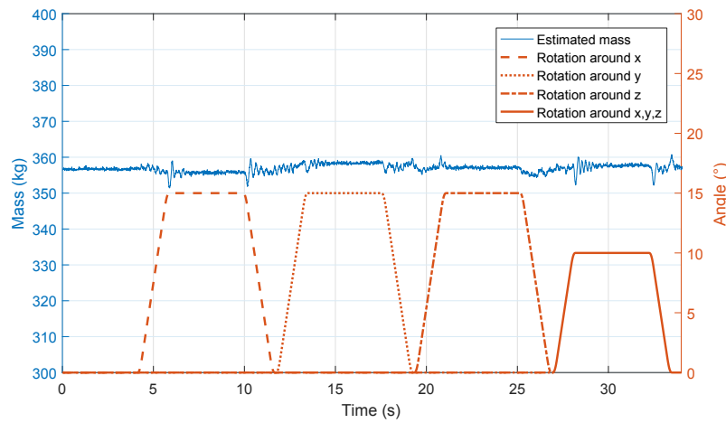
Figure 2.17: Estimated mass (kg) of MP during orientations.
