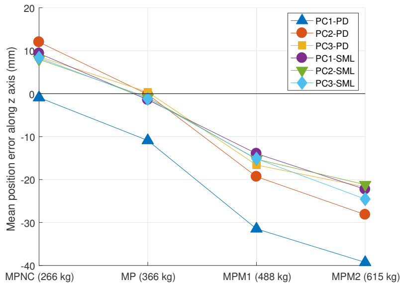
Figure 4.28: Mean position error along axis z_b for all controllers and loads (mm) for trajectory second half ( t = 30\text{s} to t = 60\text{s} )
