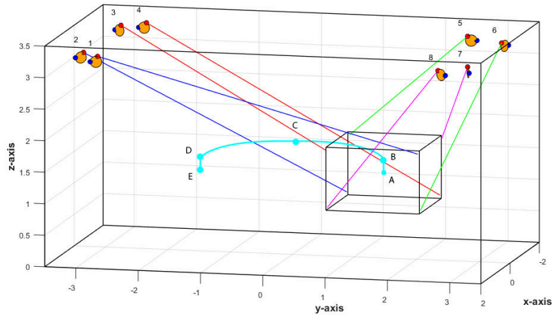
Figure 1.24: ROMP test trajectory in blue and CDPR prototype configuration with pulleys in orange.
