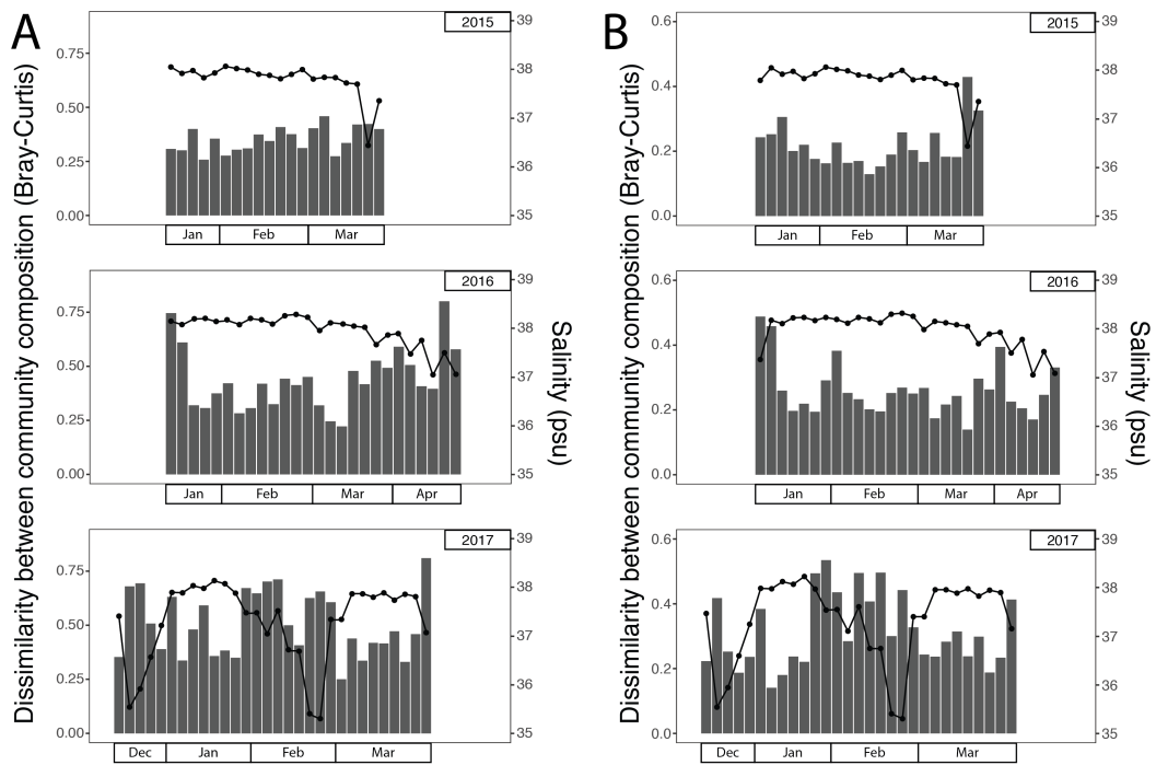
Fig. 2. : Bray-Curtis dissimilarity index between two succeeding samples, separated by year of sampling for eukaryotes (A) and prokaryotes (B). The line represents seawater salinity.
