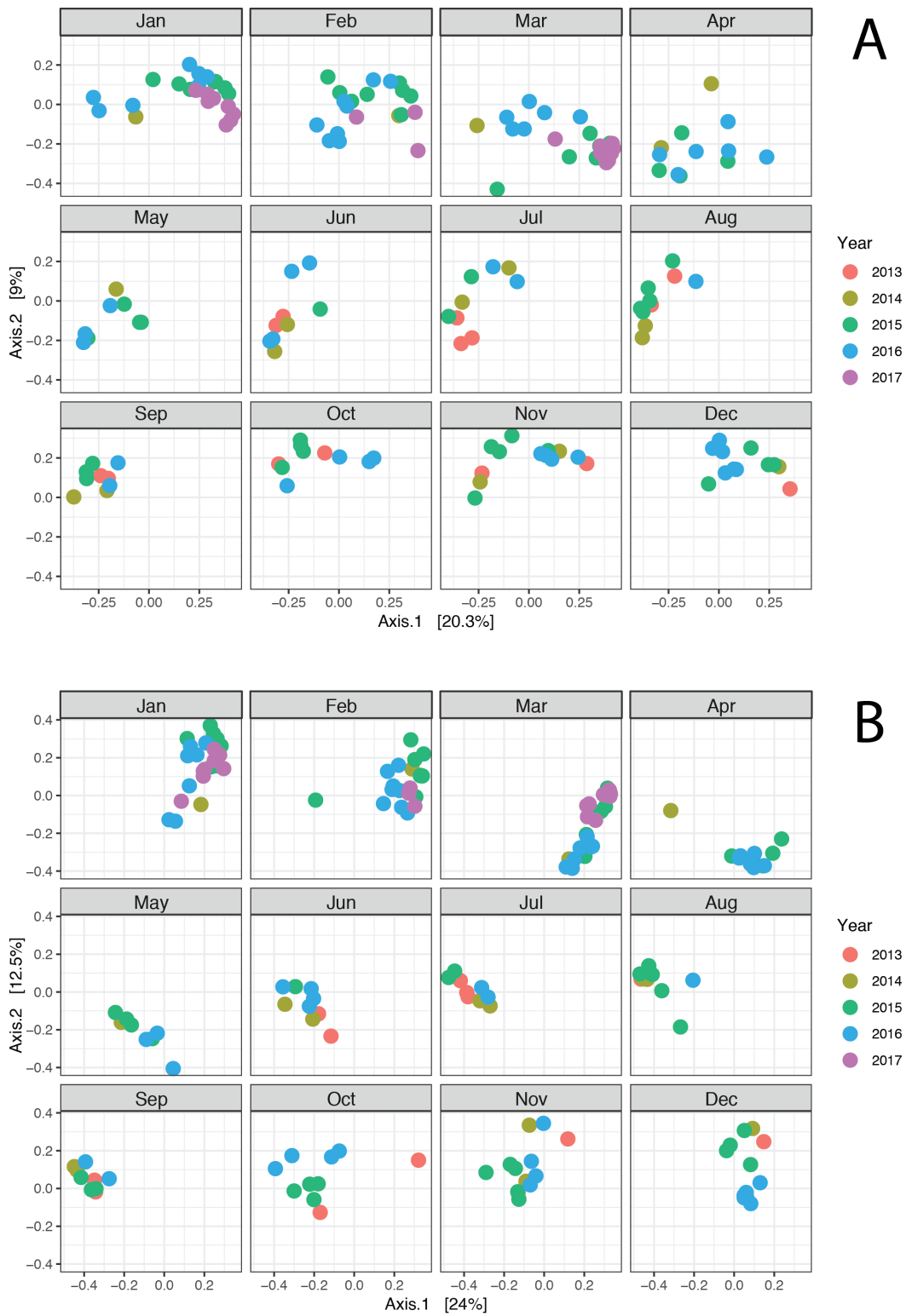
Figure 4: Principal Coordinate Analysis (PCoA) for eukaryote (A) and prokaryote community composition (B) found on 3µm filters from 2013 to 2017.
