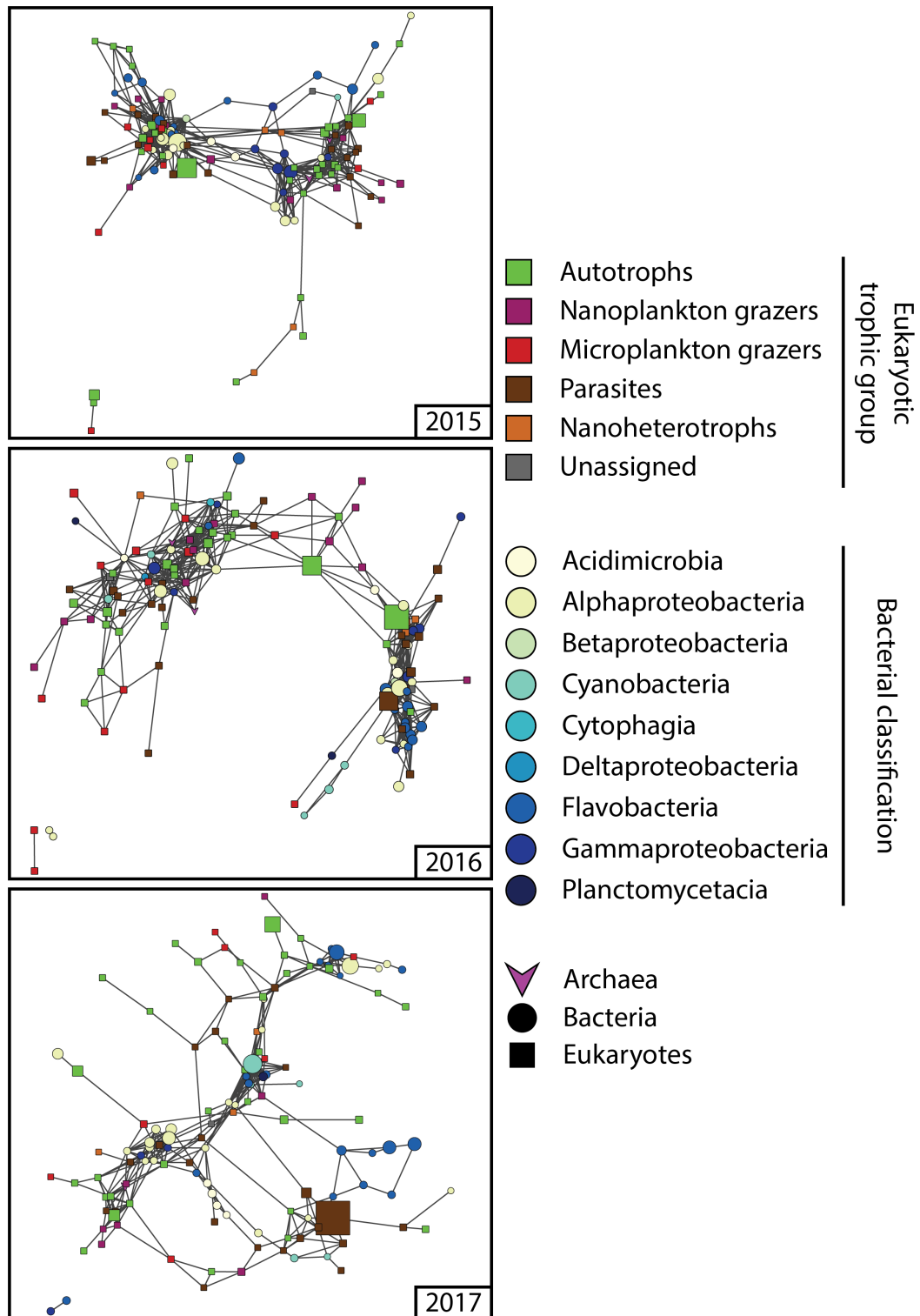
Fig. 7. : (Addendum) Yearly networks showing co-occurrences between ASVs calculated with the MIC statistic. The size of the node is proportional to the sequence abundance of its corresponding ASV. The color coding of each ASV reflects either the trophic group for eukaryotes or taxonomical classification for prokaryotes
