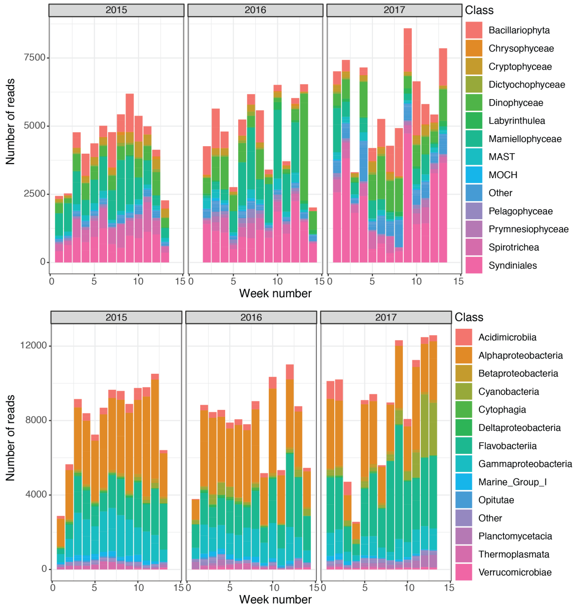
Figure 1: Number of normalized reads per year per group for Eukaryotes (top) and Prokaryotes (bottom).
