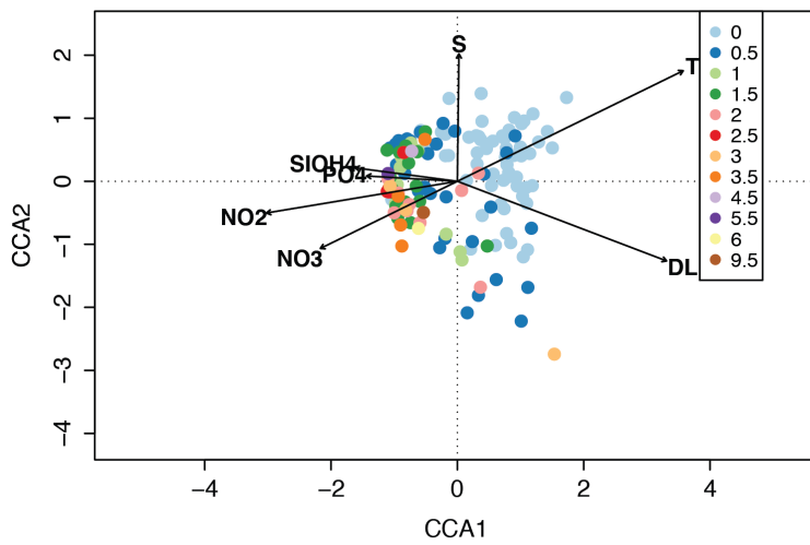
CCA of eukaryotic phytoplankton communities showing the samples month, temperature or nitrate levels
