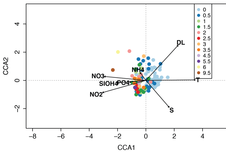
CCA of bacterial communities showing the samples month, temperature or nitrate levels
