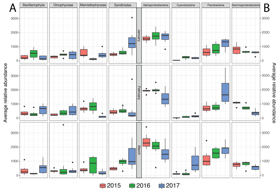
Fig. 5. : Average relative abundance of eukaryote (A) and prokaryote (B) classes according to year of sampling.
