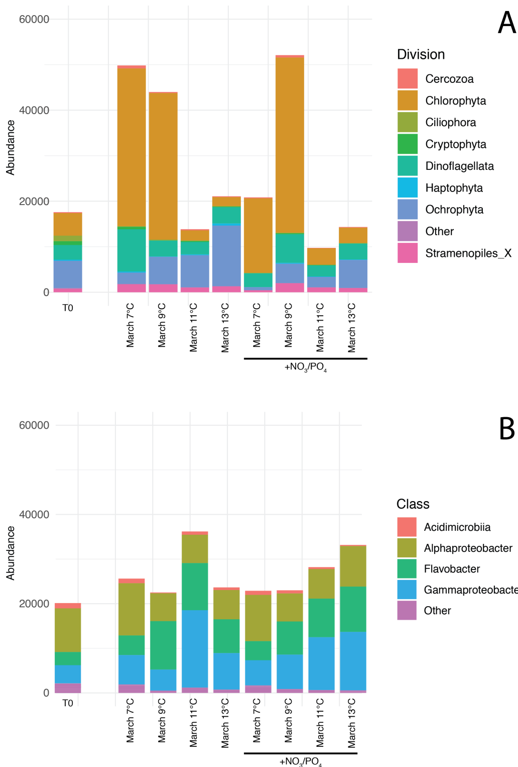
Figure 2: Sequence abundance of eukaryotes (A) and prokaryotes (B) in a microcosm experiments. T0 corresponds to starting moment of the experiment, sampled at SOLA. The legend is the taxonomy of eukaryotes at the division level and prokaryotes at the class level
