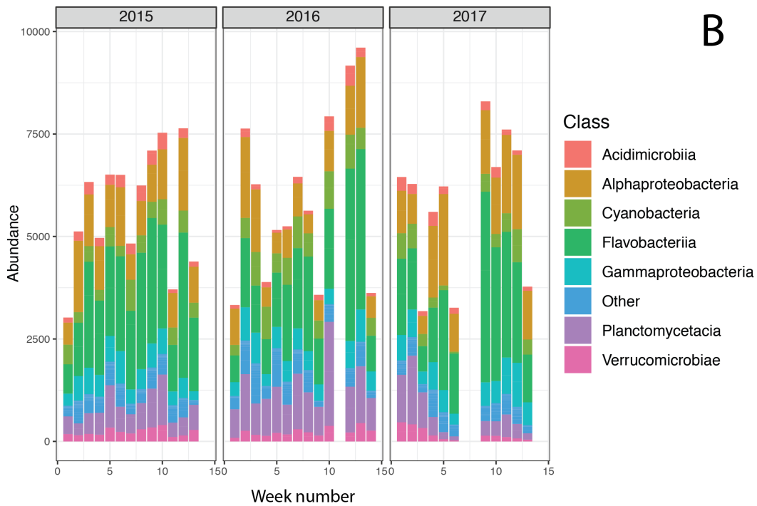
Figure 3: Sequence abundance for 3µm filters during winter from 2015 to 2017 for the eukaryotes (A) and prokaryotes (B).
