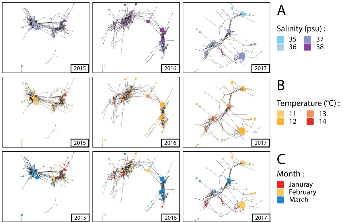
Fig. 6. : Networks showing co-occurrences between ASVs calculated with the MIC statistic. The size of the node is proportional to the sequence abundance of its corresponding ASV. The color coding of each ASV reflects either salinity (A), water temperature (B) or the month of sampling (C).
