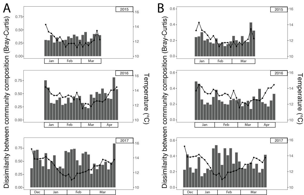
Fig. 3. : Bray-Curtis dissimilarity scores between two succeeding samples, separated by year of sampling for eukaryotes (A) and prokaryotes (B). The line represents seawater temperature.
