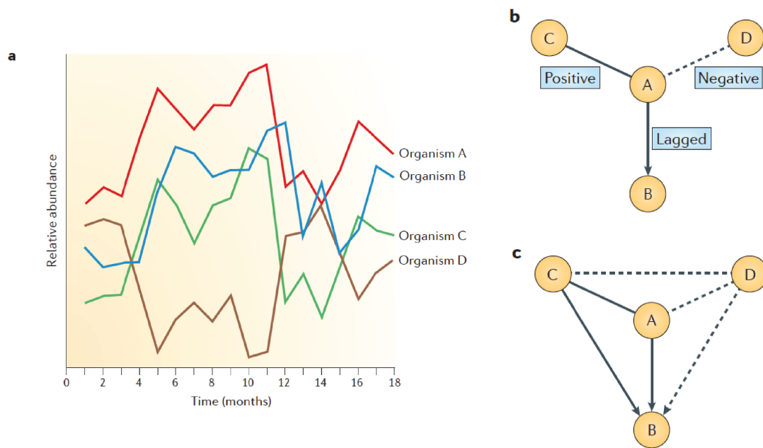
Figure 1.3: Representation of microbial interactions as a network. (a) Hypothetical abundances of four organisms over time. Organisms A and C are positively correlated, A and B as well, but with a time lag of one month and A and D are negatively correlated. (b) The previously described correlations are then translated into a network. (c) Using the previous nomenclature (from (b)), this network describes all the correlations between the four hypothetical organisms (59).
