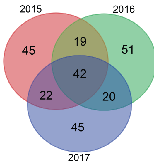
Fig. 8. : Venn diagram showing the shared and/or specific eukaryotic and bacterial ASVs per year.
