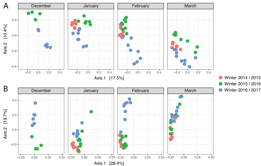
Fig. 4. : Principal Coordinate Analysis (PCoA) for eukaryote (A) and prokaryote community composition (B).
