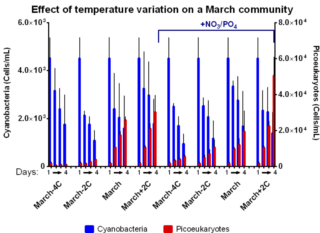
Figure 1: Cell density for picoeukaryotes and cyanobacteria during a 4 day incubation in a light and temperature controlled microcosm. Temperature variations were tested on natural communities in normal or enriched conditions.
