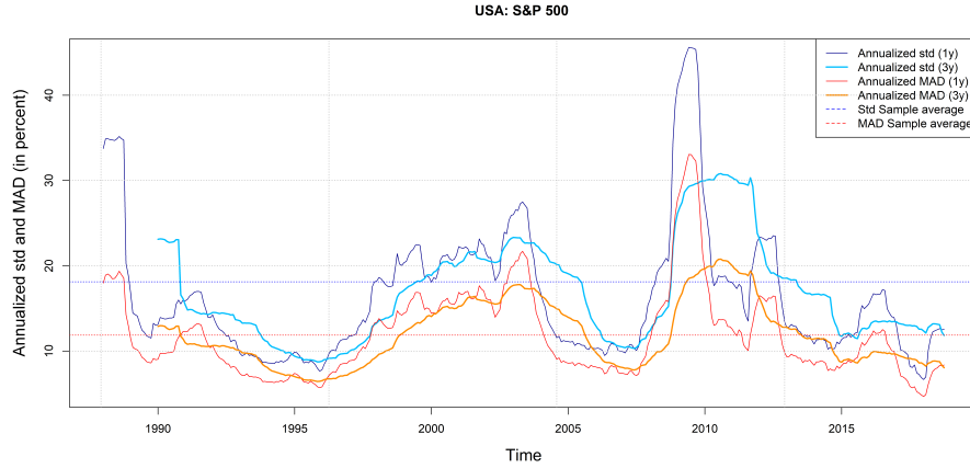
FIGURE 2.2: Annual realized volatility v_{k,T}(t) , defined in (2.9), in percent, for k = 1 (MAD) and k = 2 (std), of the S&P 500 returns over a rolling sample of size T = 1, 3 year(s). The dashed lines represent the sample average (over the whole sample) of the two different measures of the volatility (with the same color code).
