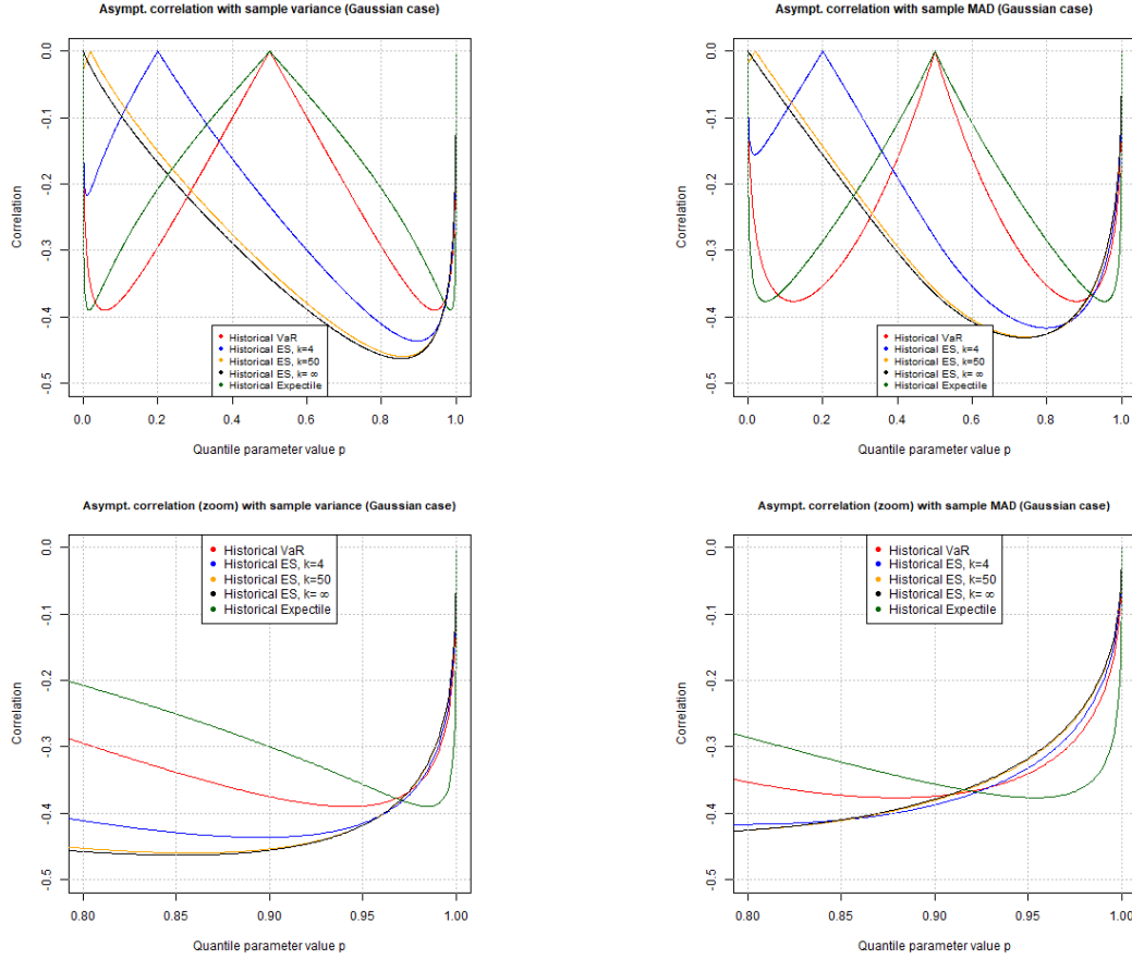
FIGURE 5.1: Pro-cyclicity as defined in (5.10), considering on each plot three different risk measures (VaR, ES, evaluated in 3 possible ways, and expectile). In the left column the measure of dispersion is the sample variance, in the right column the sample MAD. Case of an underlying Gaussian distribution.
