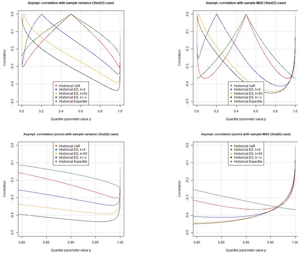
FIGURE 5.2: Pro-cyclicity as defined in (5.10), considering on each plot three different risk measures (VaR, ES, evaluated in 3 possible ways, and expectile). On each row in each plot a different measure of dispersion is considered (from left to right: sample variance, sample MAD. Case of a Student distribution with 5 degrees of freedom.
