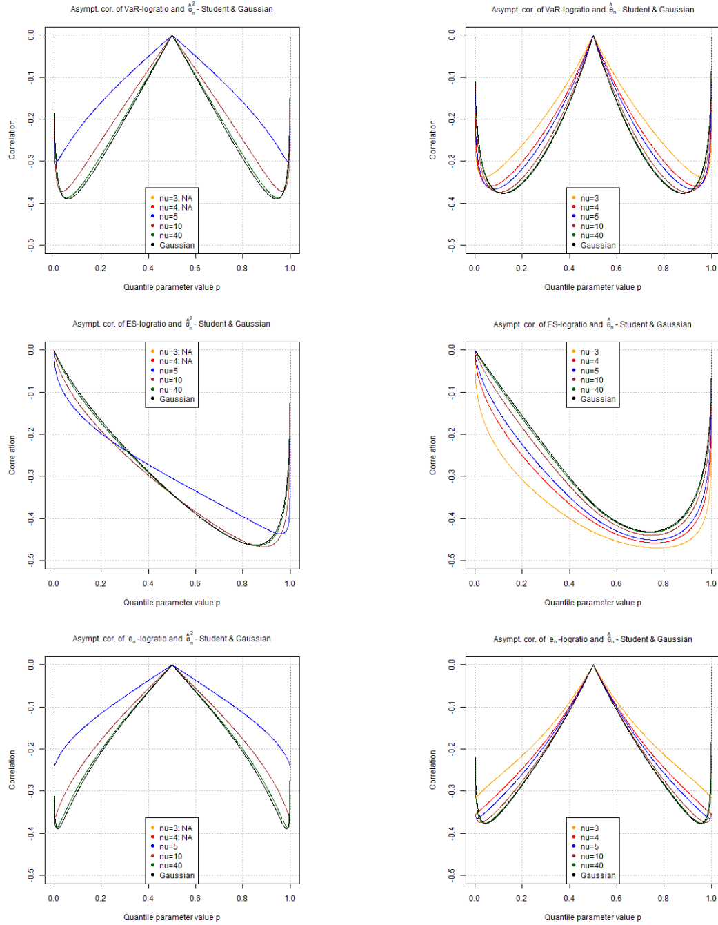
FIGURE 5.3: Pro-cyclicity as defined in (5.10), comparing the case of a Student distribution -with \nu = 3, 4, 5, 10 and 40 degrees of freedom as well as the Gaussian distribution. From top to bottom: sample quantile, ES, expectile; and from left to right: sample variance, sample MAD.
