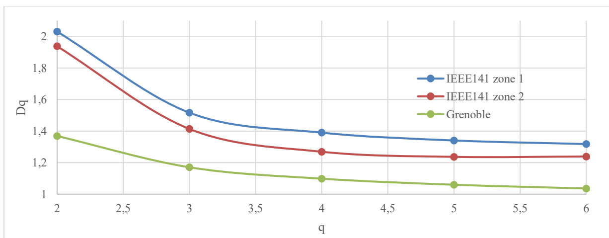
Figure 4-17: Generalized dimension for voltage drops
