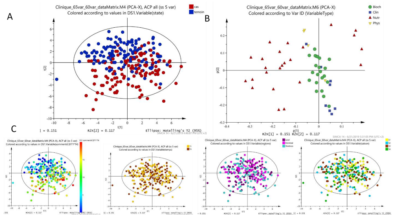
Figure 2: Principal component analysis derived from the 22 biochemical parameters, 9 variables from clinical examination, and 4 scores in link with physical activity, and 25 nutritional data considered from the 123 studied subjects. A: score plot (PC1: 15.1% of variance; PC2: 11.7% of variance); B: loading plot (PC1-PC2); C: projections of main confounding factors of the study design.
