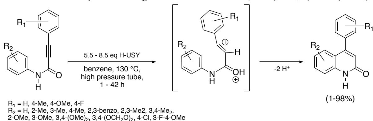
Scheme 40: The intramolecular cyclization of N -aryl of 3-arylpropynamides under the action of H-USY zeolite
