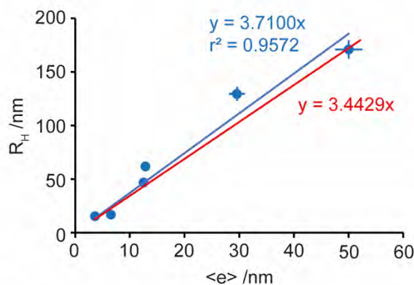
Figure 20. Correlation between the mean R_H obtained by DLS and \langle e \rangle (in blue) compared to the predicted correlation (in orange) for talc nanoparticles at equilibrium morphology in presence of water.
