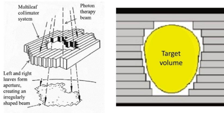
Figure 1.4 Schematic of multileaf collimator (source:[17]); Individually positioned leaflets shape the beam to the target
