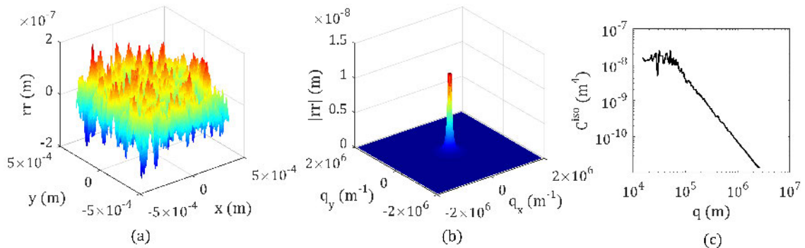
Figure 4.4: The selected artificial surface roughness (a), amplitude distribution of this surface roughness (b) and its power spectral density (c).
