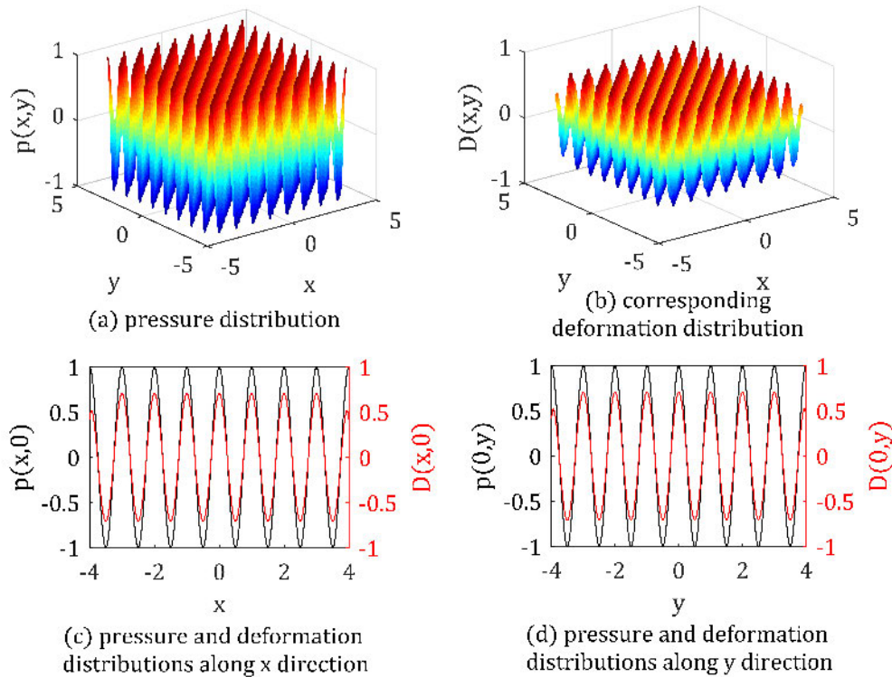
Figure D.1: Pressure distribution and the corresponding elastic deformation.
