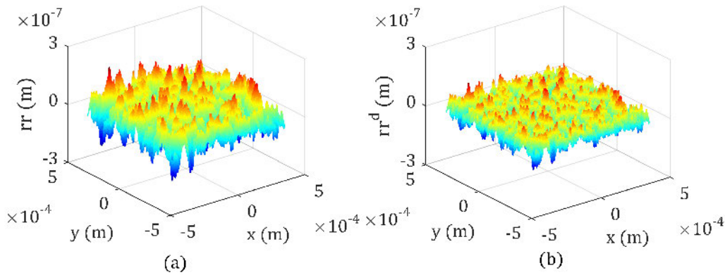
Figure 4.6: Comparison between the initial surface roughness (a) and the deformed surface roughness (b).
