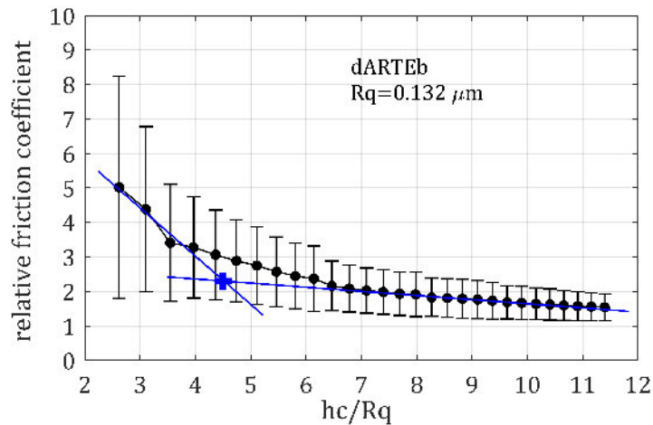
Figure 4.31: The relative friction coefficient as a function of the " \Lambda ratio" for the surface roughness dARTEb.
