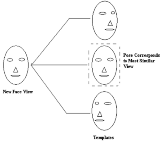
Figure 2.2: Appearance Methods
