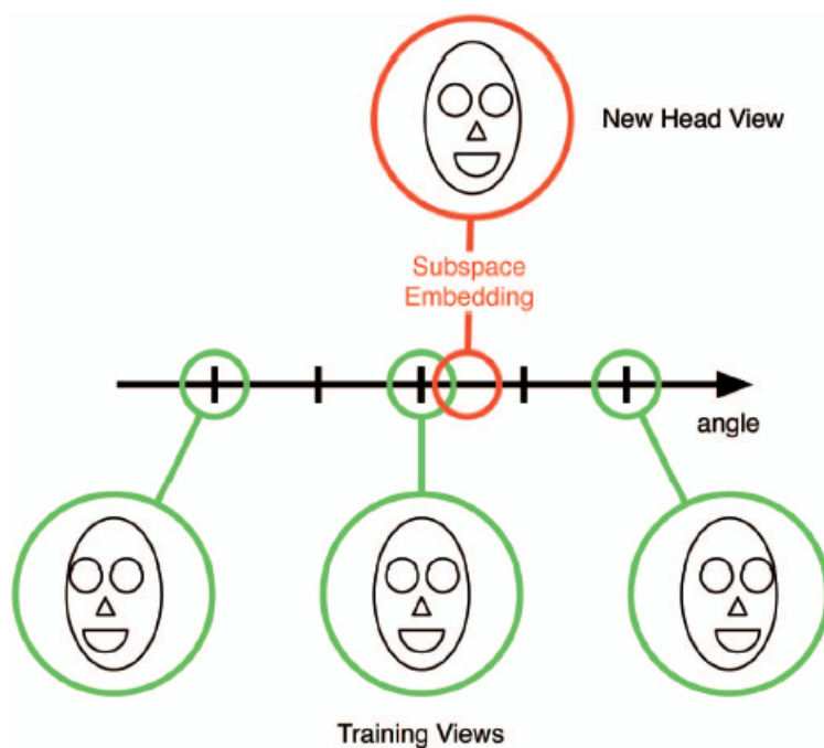
Figure 2.4: Manifold Methods
