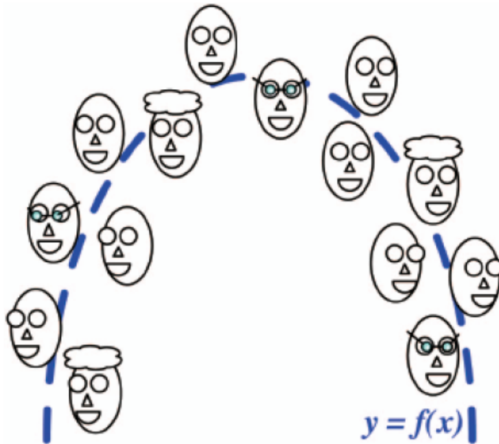
Figure 2.3: Regression Methods
