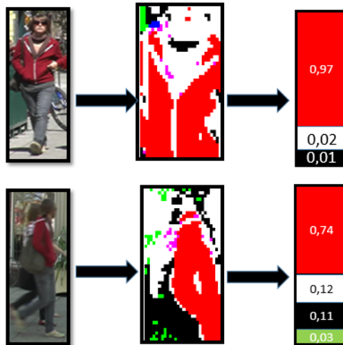
Figure 3: Color Categorisation
