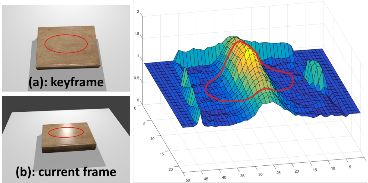
Fig. 2.5 The illumination variation in the image plane between the keyframe K and the current frame F is viewed as an elevation map. In this example, a specularly crosses the target region \mathcal{T}_F . This demonstrates the smoothness and continuity properties of a specularly.
