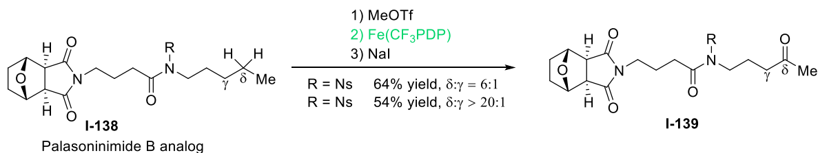
Scheme I-13 Innate C-H oxidations
