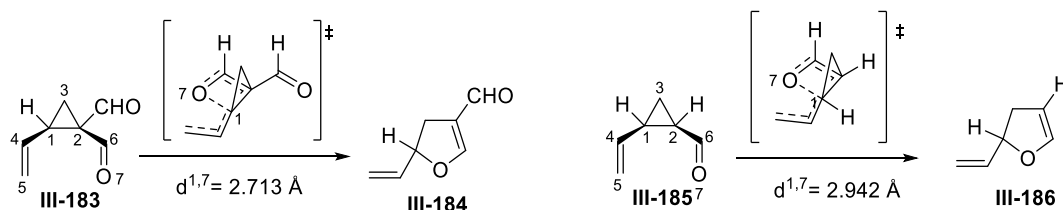
Scheme III-49 Substituent effects of [1,3]-sigmatropic rearrangement (reaction B)
