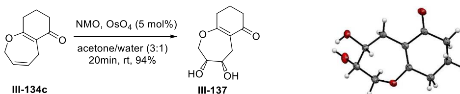
Scheme III-32 Structural confirmation of 2,5-dihydrooxepine
