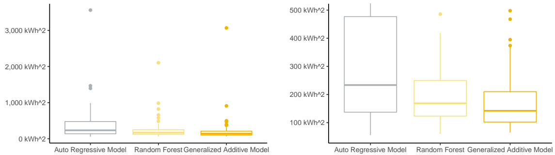
Figure 11 – Distribution over the test period of daily mean squared error of global consumption benchmark forecasts (auto-regressive model, generalized additive model, random forest). Left picture: original boxplots; Right picture: boxplots trimmed at 500 \text{ kWh}^2 .
