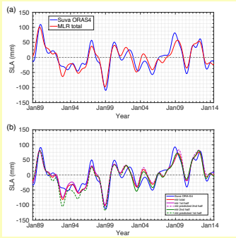
Figure 4: ORAS4 and curl_2 \tau dominated MLR modeled sea-levels over the 1988-2014 period for the Suva site (a) detrended, (b) trends included, with stationarity test results
