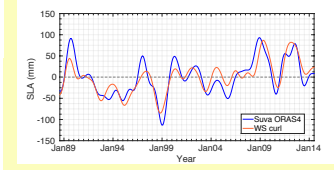
Figure 5: ORAS4 sea-level and curl_2 \tau regressor timeseries over the 1988-2014 period for the Suva site (from Figure 4), plus comparison metrics
