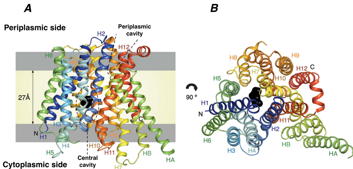
Figure 25. Global structure of PepT so .
