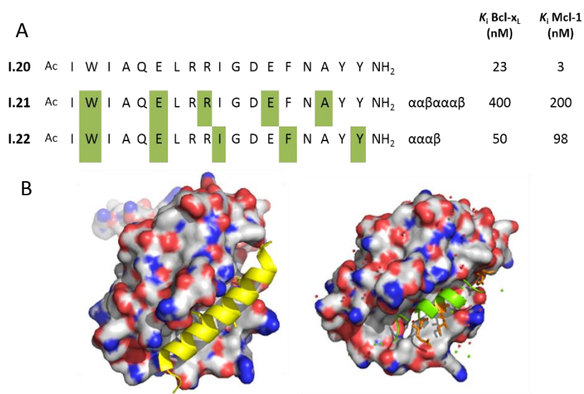
Figure 17: Sequence of natural peptide and two \alpha/\beta peptide mimics and crystal structure of one \alpha/\beta peptide in complex with Bcl-x L . A) Sequences of natural peptide I.20 and \alpha/\beta peptide I.21 and I.22 . \beta^3 -Residues are highlighted in green. B) Crystal structure of Bim BH3 peptide (yellow) in complex with Bcl-x L (pdb entry: 3FDL). The crystal structure of the compound I.22 (green) in complex with Bcl-x L reveals the same surface of contact as the one of the natural peptide is involved in the interaction (pdb entry: 4A1W).
