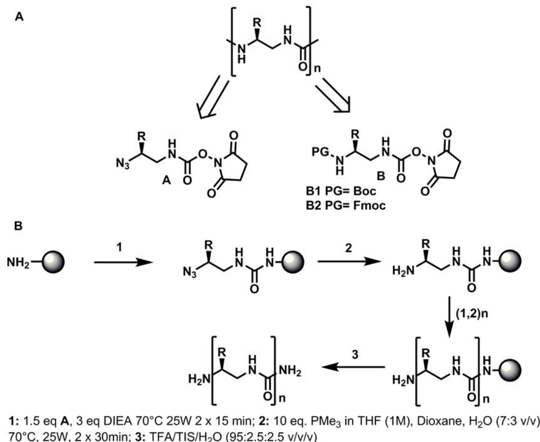
Figure 39: A) Schematic representation of oligourease and formulas of azide monomers A and activated protected monomers B. B) Scheme of the solid phase synthesis approach under microwave assistance with the most recent azide strategy.
