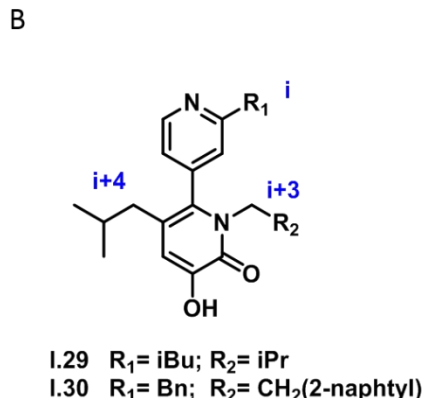
Figure 20: X-ray crystal structure of ER ligand binding domain in complex with peptide GRIP1 coactivator and trisubstituted biaryl scaffold developed by Hamilton and coll. A) X-ray crystal structure of ER ligand binding domain (blue) in complex with peptide GRIP1 coactivator \alpha -helical peptide (yellow) (PDB entry: 3ERD) B) Chemical structure of pyridylpyridone derivatives 1.29 and 1.30 mimicking i , i +3 and i +4 residues of the \alpha -helix.
