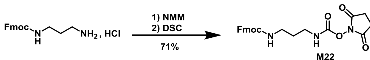
Scheme 24: Synthesis of Fmoc-DAP u -OSu (M22) in CH 2 Cl 2
