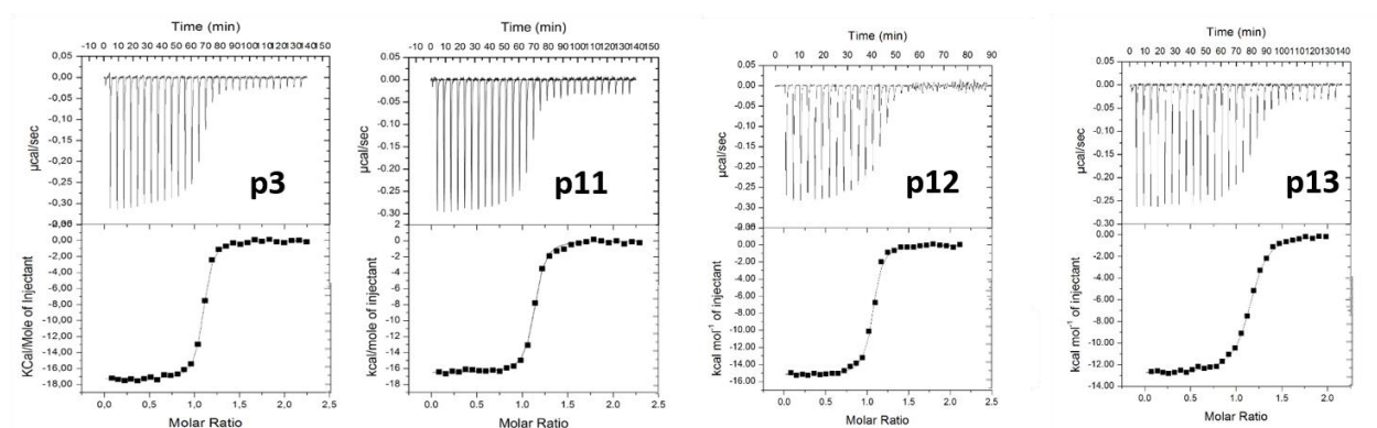
Figure 82: The binding parameters (affinity constant K_D , stoichiometry N, binding enthalpy \Delta H , entropy -T\Delta S and free energy \Delta G ) of p11-p13 determined during ITC measurements
