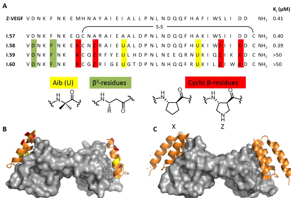
Figure 25: Presentation of Z-VEGF 1-38 \alpha and \alpha/\beta -peptides A) Primary sequences of \alpha and \alpha/\beta -peptides with non-natural peptides in color with their chemical structure. B) Crystal structure of I.58 (orange) in complex with VEGF (grey) (PDB 4WPB). C) Crystal structure of Z-VEGF (orange) in complex with VEGF (grey) (PDB 3S1K).
