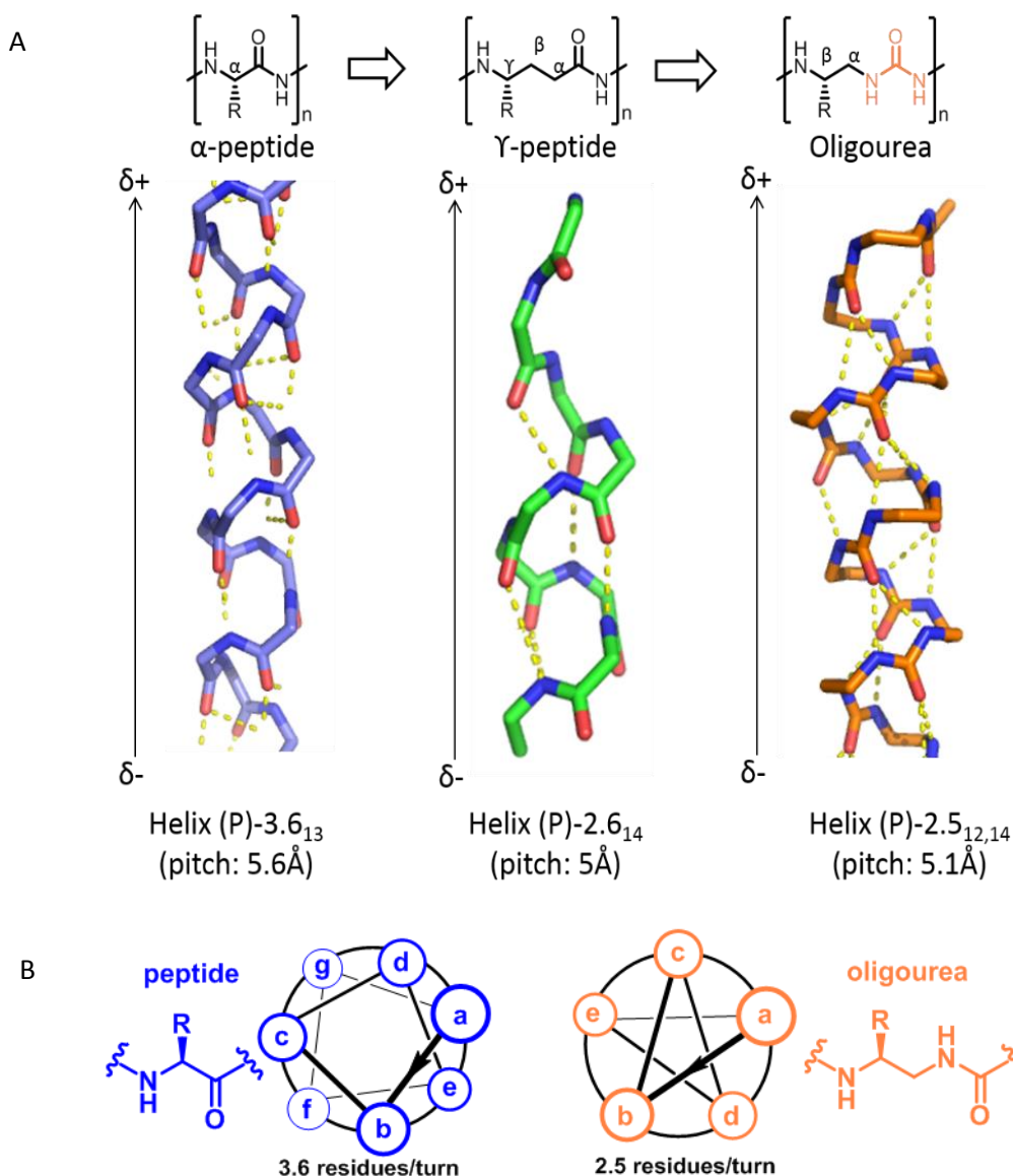
Figure 38: Comparison of foldamer helical structures with the \alpha -helix. A) Structure of \alpha -peptide (in blue), Y-peptide (in green) and oligourea (in orange) without side chains B) Diagram wheels of peptide in blue and oligourea in orange.
