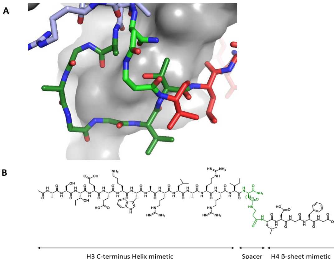
Figure 81: Design of a shorten linker to bypass the GAGG segment. A. Model design of the spacer (light green) on the X-ray crystal structure of p3-Asf1. B. Chemical structure of compound designed with the variable number of methylene units n = 1 or 2 .
