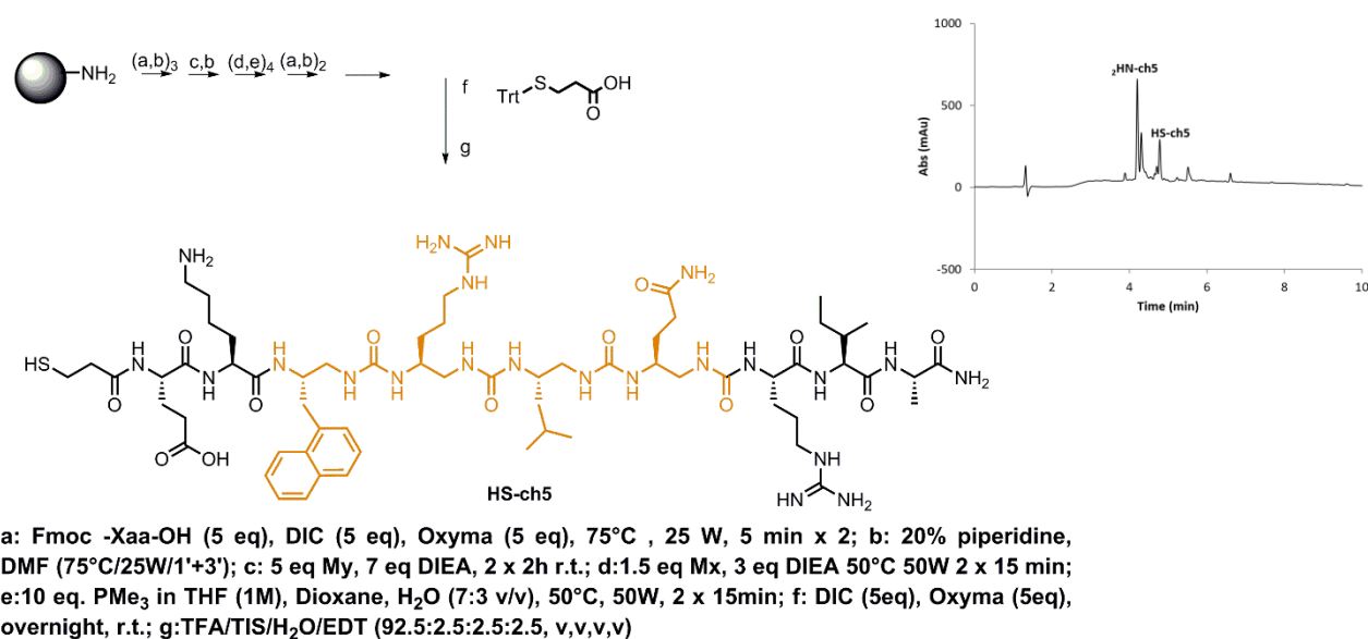
Scheme 17 : Solid phase synthesis of HS-ch5 and its HPLC chromatogram
