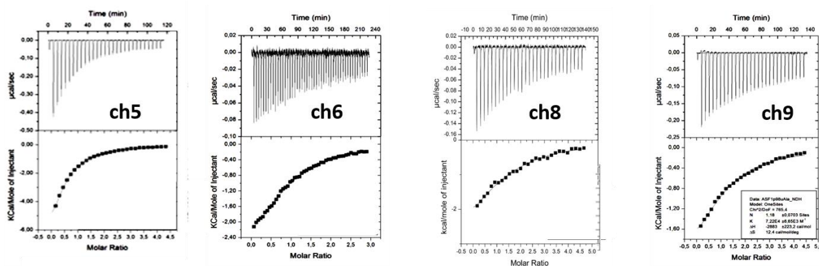
Figure 61: Thermodynamic data of compounds ch5-ch9 measured by ITC. ITC curves of ch5, ch6, ch8 and ch9 and fitted curves are shown. Experiments were carried out at 20°C, in a 50mM Tris-HCl pH7.4
