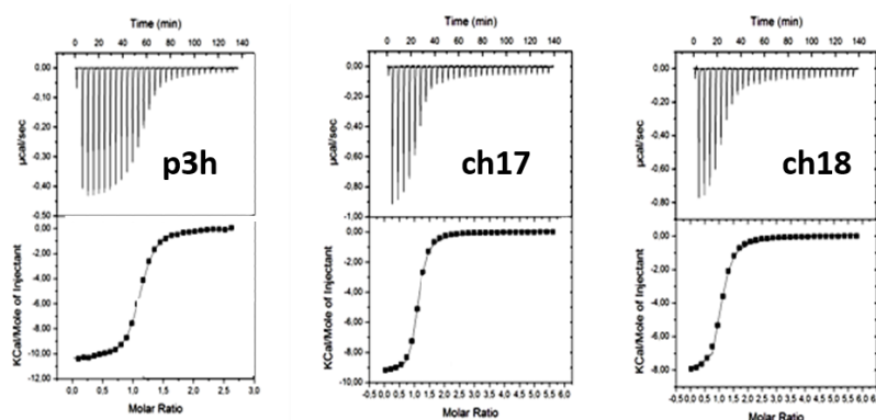
Figure 71: Thermodynamic data of compounds ch17-ch19 measured by ITC experiments. ITC curves of p3h , ch17 - ch18 and fitted curves are shown. Experiments were carried out at 20°C, in a 50mM Tris-HCl pH7.4
