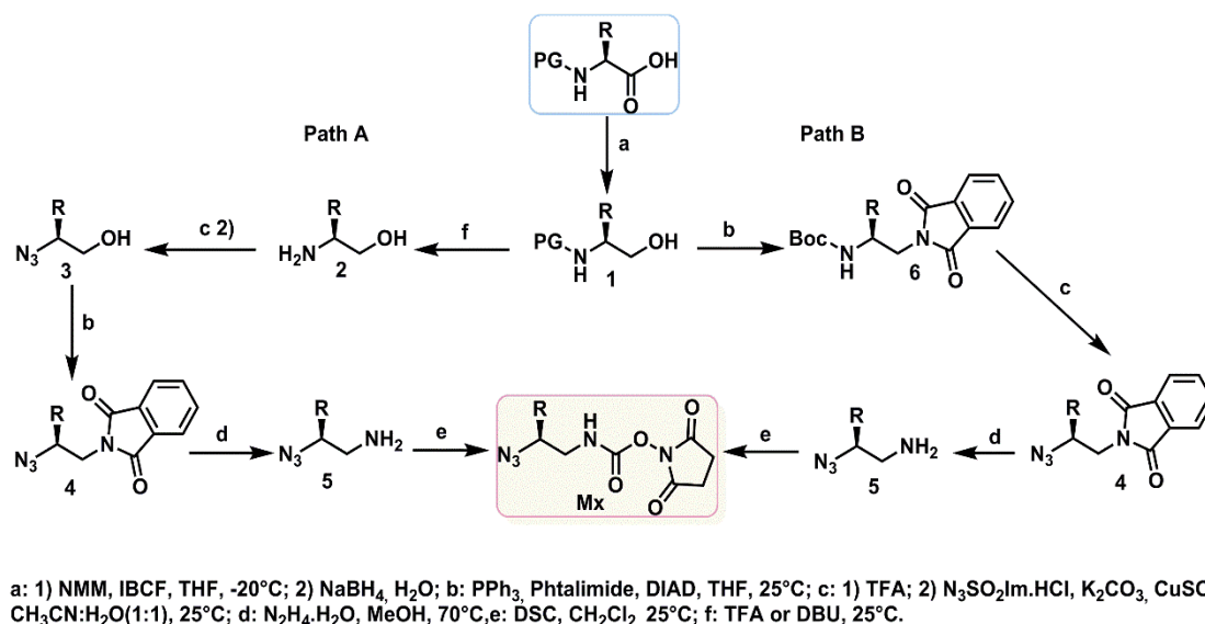
Scheme 2: General procedure for the preparation of succinimidyl (2-azido-2-substituted ethyl) carbamate (azide monomers) Mx with two routes depending on the nature of the side chain.
