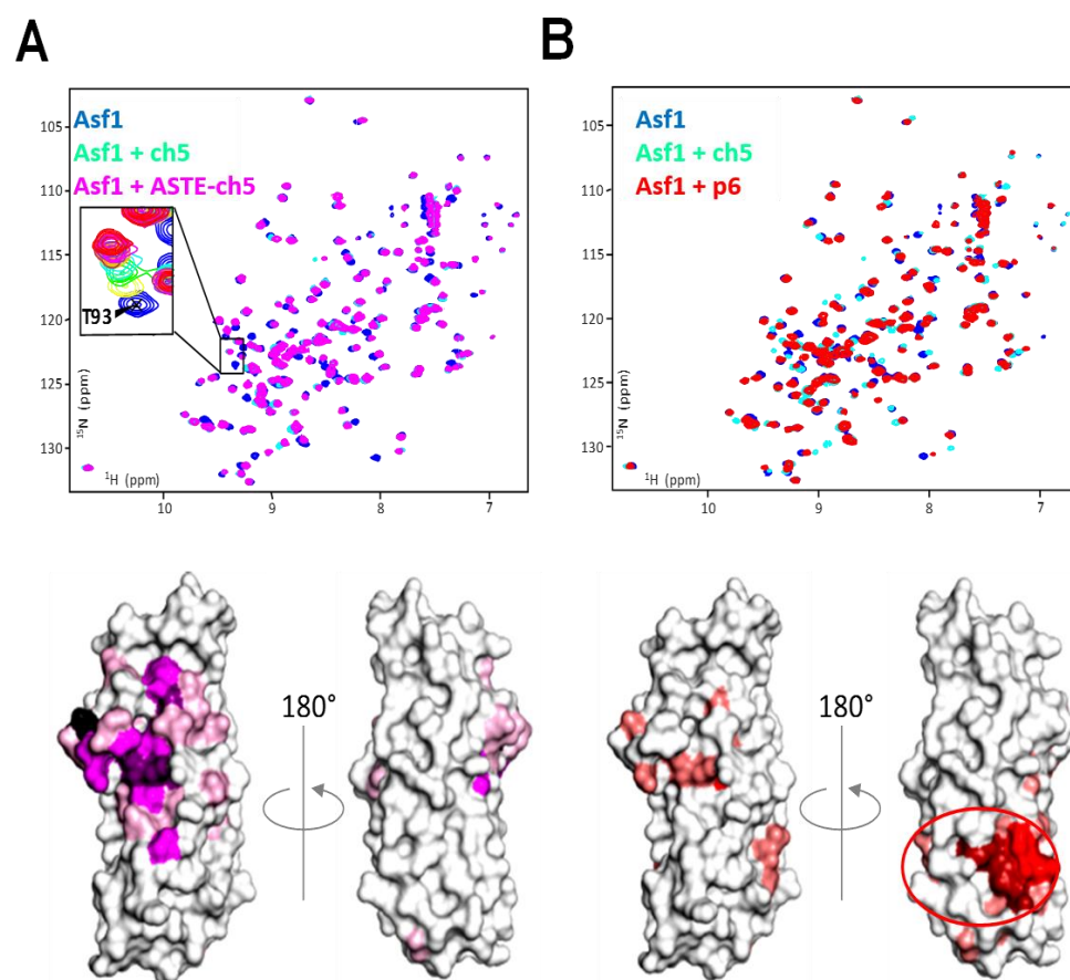
Figure 64: Comparative HSQC analysis of ch5 , ASTE-ch5 and p6 . A and B, upper panels, overlay of NMR ^1\text{H} - ^{15}\text{N} HSQC spectra corresponding to the free Asf1 (blue), ch5 -bound (cyan), ASTE-ch5 -bound (A) (magenta), or p6 -bound (B) (red) forms of Asf1. Spectra were recorded at 25°C, in Tris 10mM buffer pH7.5, before and after addition of an excess
