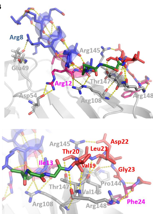
Figure 76: Interactions observed into the complex between Asf1 and p3. A List of Asf1 residues interaction with p3 residues. B X-ray crystal structure of the complex with zoom on H-bonds involved for the stabilization of the complex.
