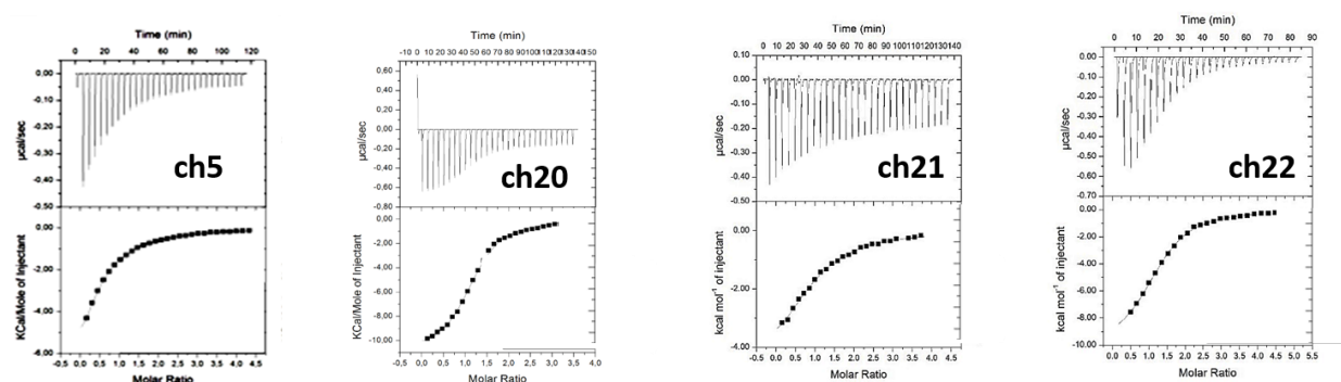
Figure 85: The binding parameters (affinity constant K_D , stoichiometry N, binding enthalpy \Delta H , entropy -T \Delta S and free energy \Delta G ) of ch20-ch22 determined during ITC measurements
