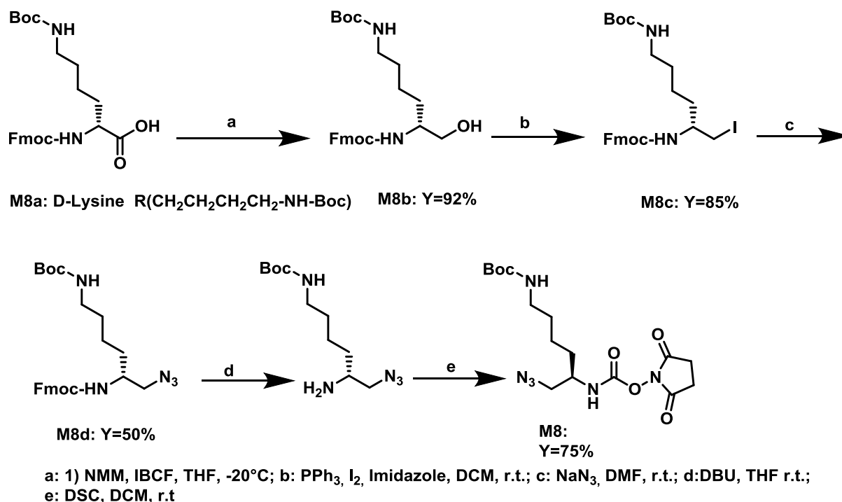
Scheme 6: The synthesis of succinimidyl (2-azido-1-substituted ethyl) carbamate M8 , bearing a shifted lysine side chain
