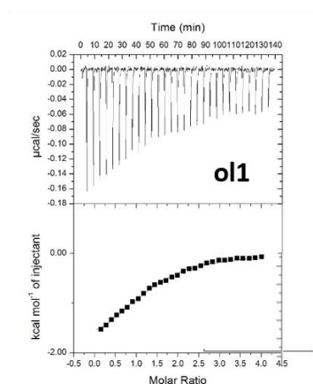
Figure 74. Thermodynamic data of compound ol1 measured by ITC experiments. ITC curves of ol1 and fitted curves are shown. Experiments were carried out at 20°C, in a 50mM Tris-HCl pH7.4
