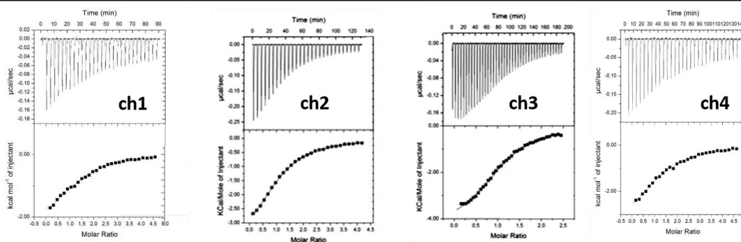
Figure 59: Thermodynamic parameters of compounds ch1-ch4 measured by ITC. ITC curves of ch1-ch4 and fitted curves are shown. Experiments were carried out at 20°C, in a 50mM Tris-HCl pH7.4
