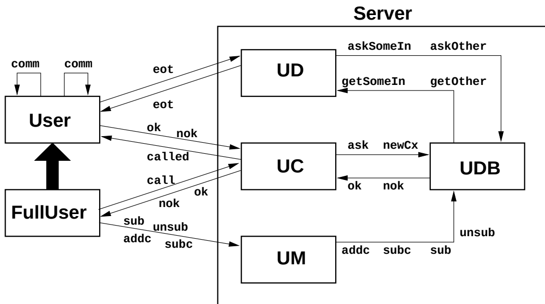
Figure C.26 : Messagerie – Composition
