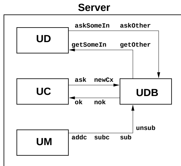
Figure C.24 : Serveur – Composition
