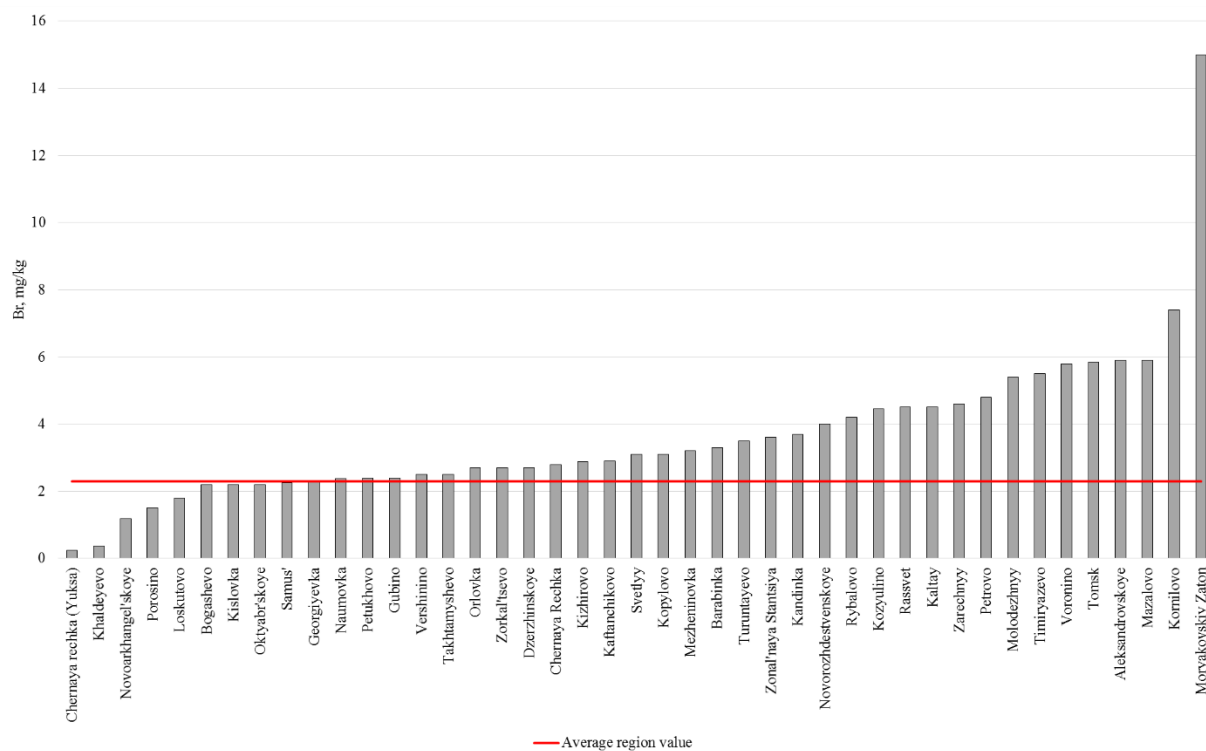
Figure 7.6 - Ranking of settlements of the Tomsky district according to the Br content in the scale of drinking water, mg/kg
