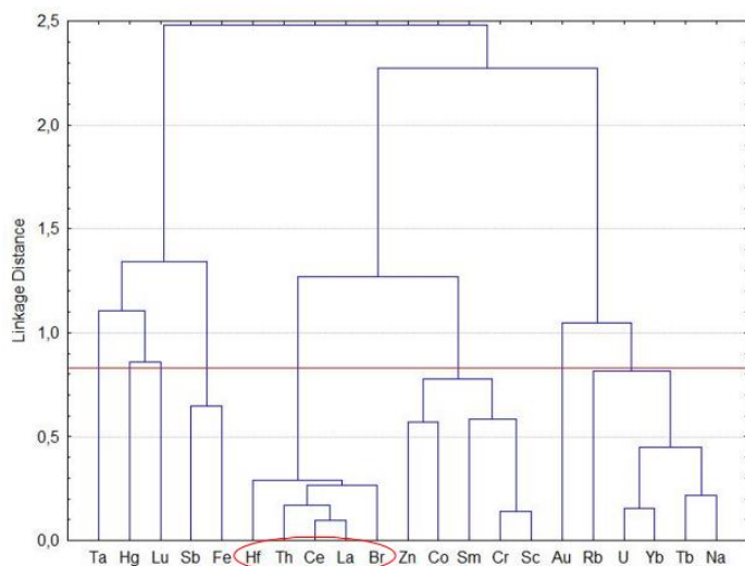
Figure 7.16 - Dendrogram of the correlation matrix of the geochemical spectrum of elements in the blood of the Tomsky district residents (1-Person r(0.05) = 0.83 , sample size - 133 samples)
