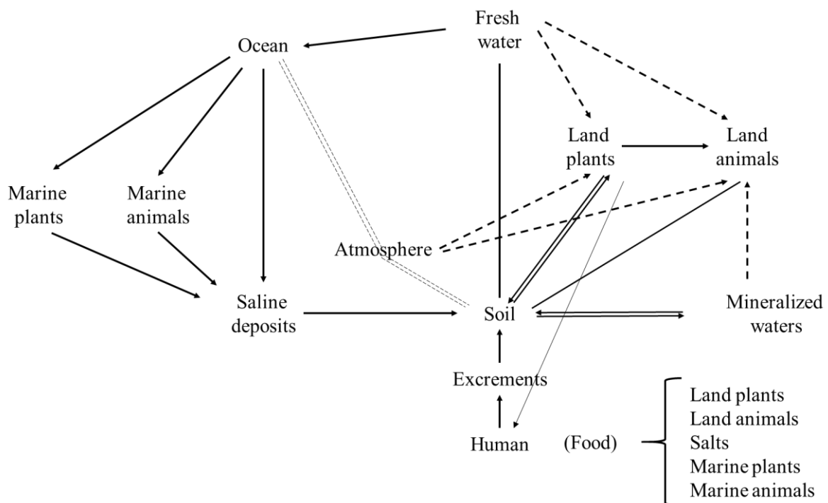
Figure 2.1 – Bromine cycle in nature ( Rosen, 1970 )
